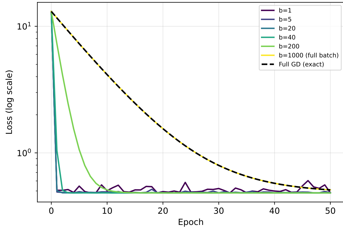
Q2: SGD Convergence vs Batch Size ( \sigma = 1 , 50 epochs)
