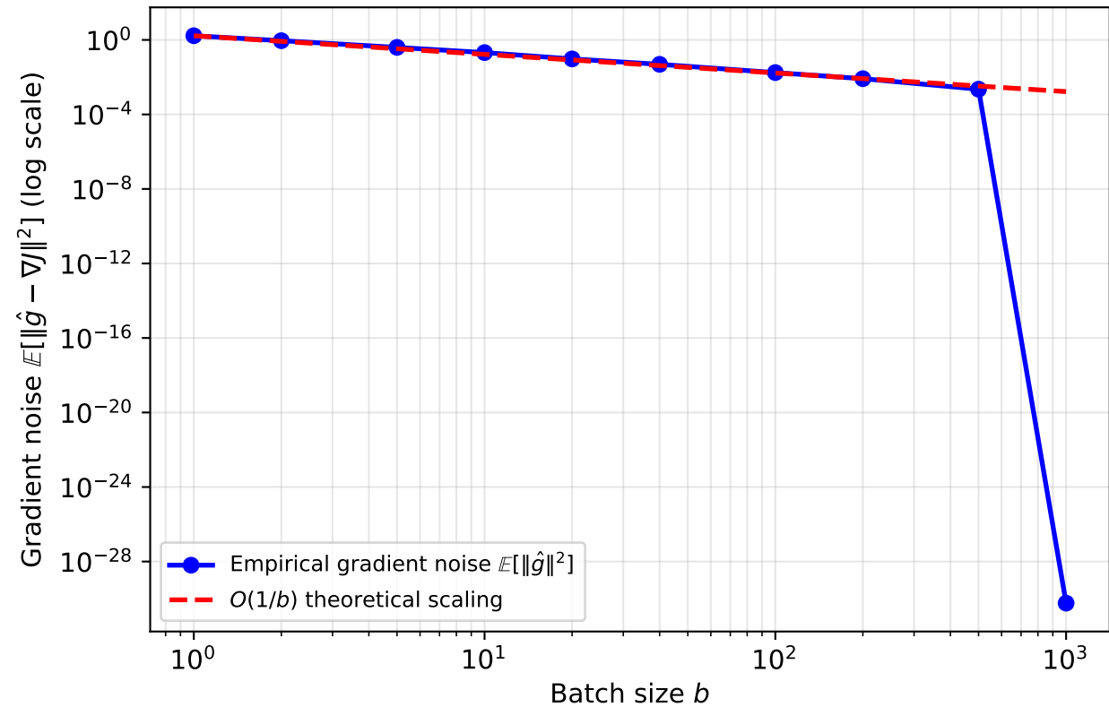
Q2: SGD Gradient Noise vs Batch Size at Optimum
