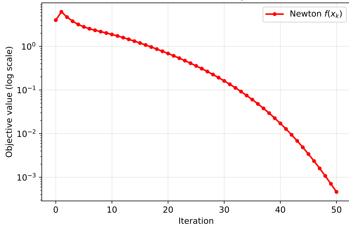
Newton's Method on Rosenbrock: Objective vs Iteration
