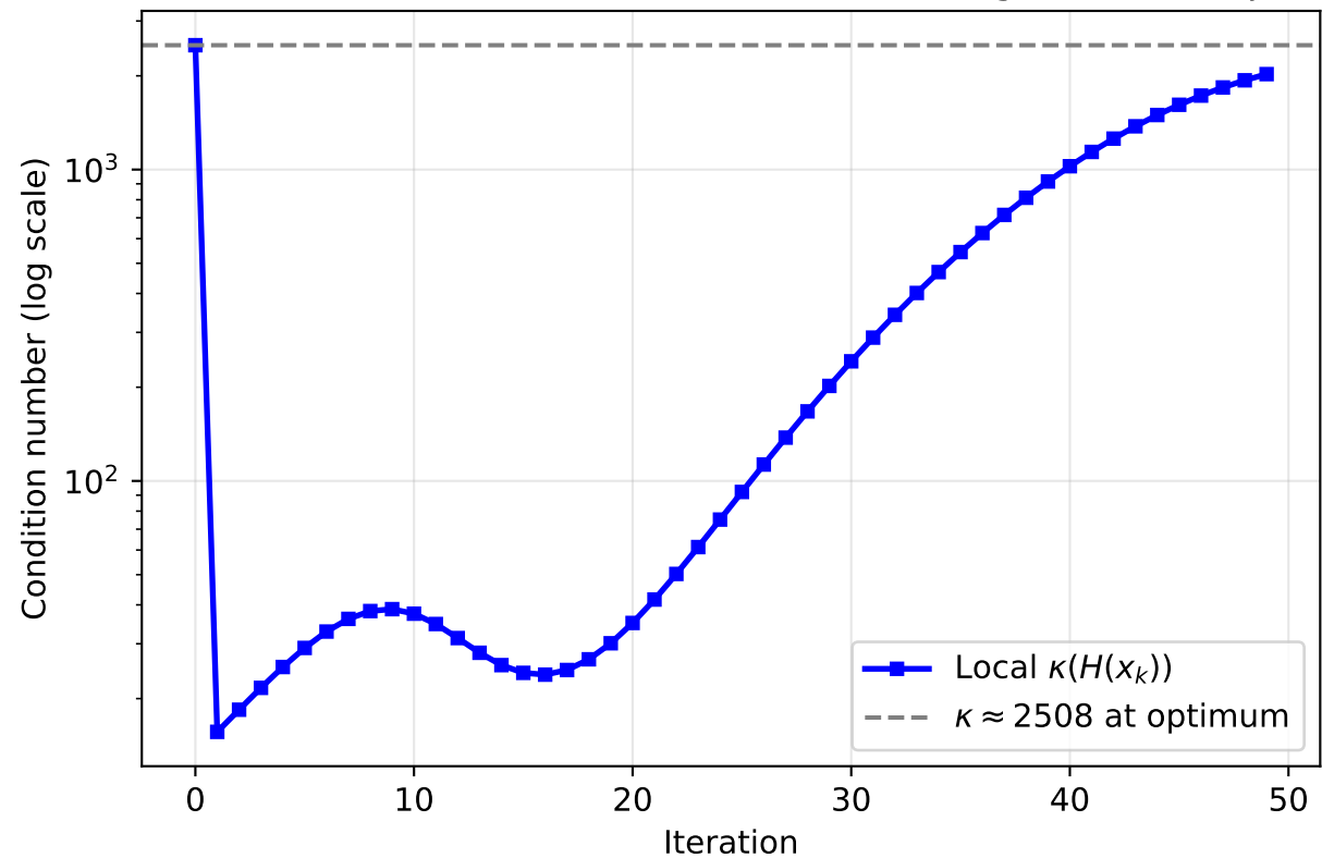
Local Hessian Condition Number \kappa(\nabla^2 f(x_k)) Along Newton Trajectory
