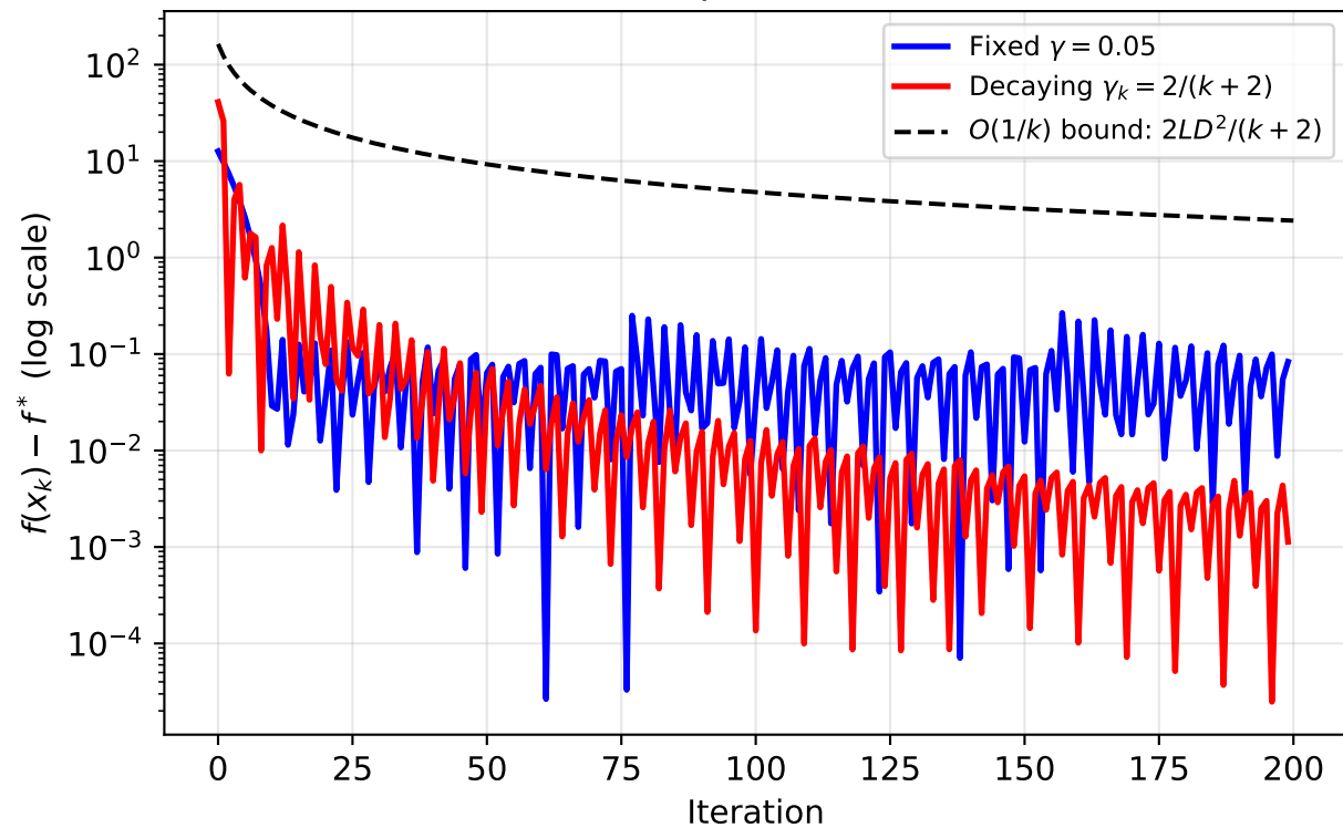
Q6: Fixed vs Decaying Step Size in Frank--Wolfe (Interior optimum, f^* = 0 )
