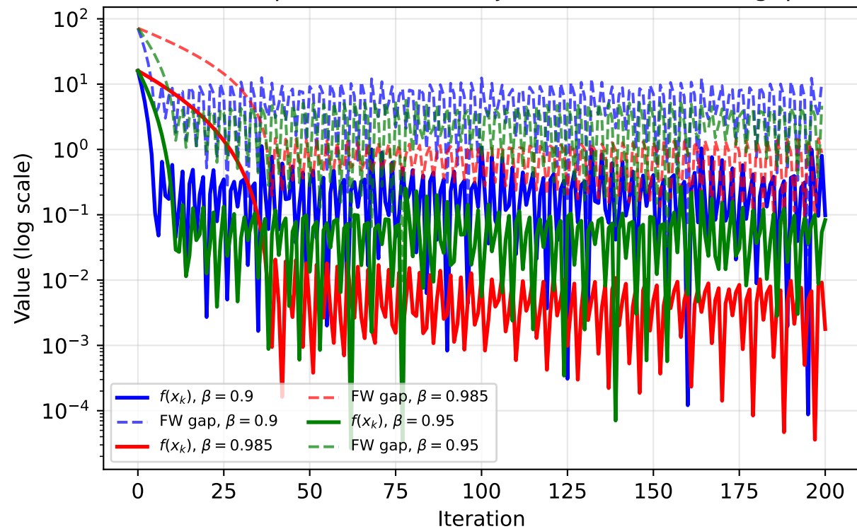
Q6: FW Objective and Duality Gap vs Iteration (Interior optimum, solid=objective, dashed=FW gap)
