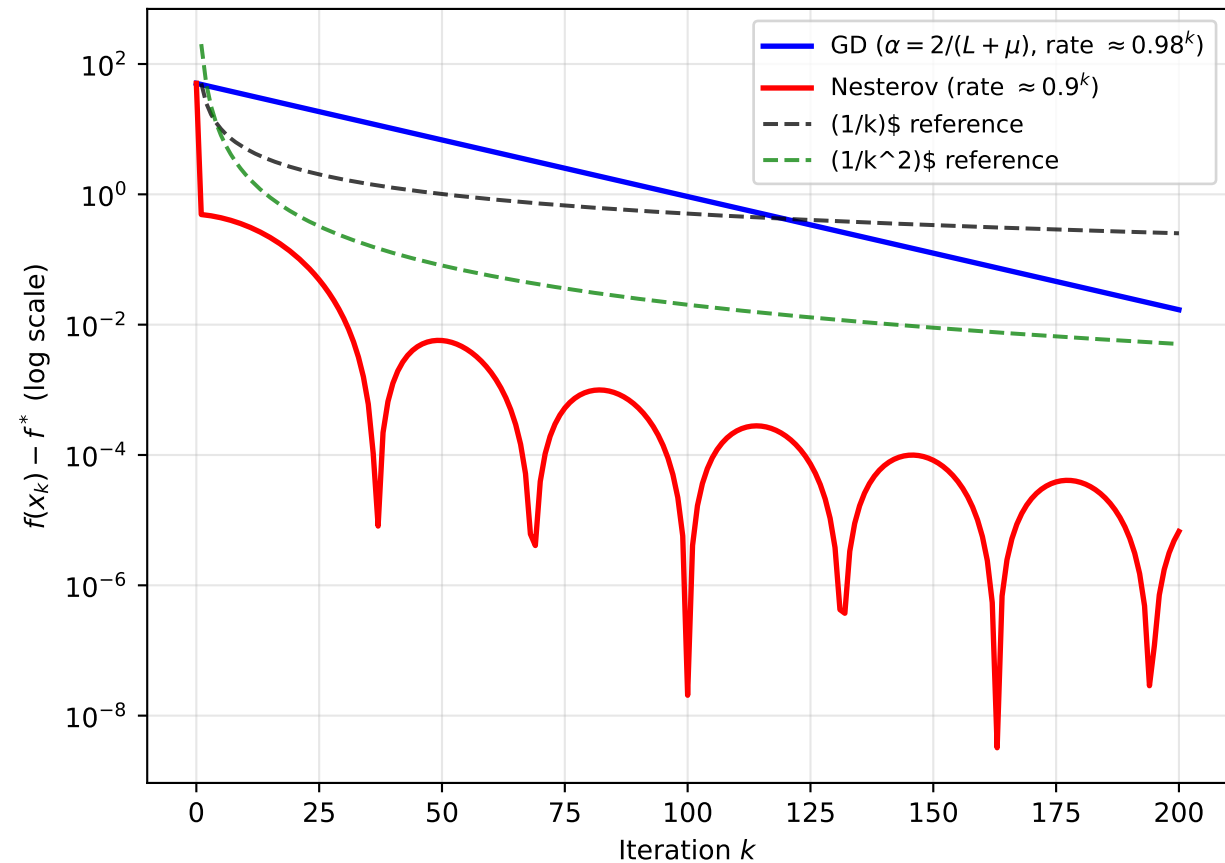
Strongly convex quadratic ( \kappa = 100 ): semi-log
