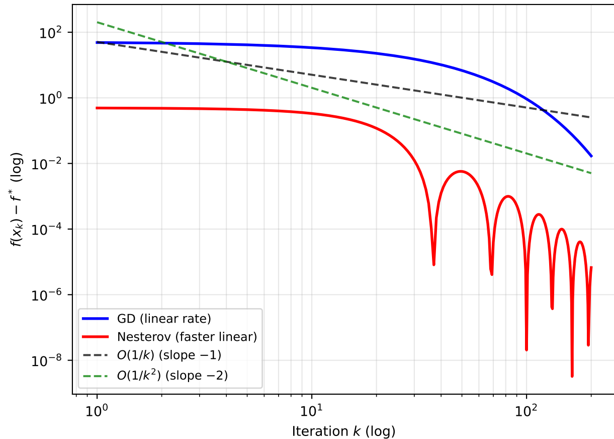
Log-log: linear vs polynomial reference rates
