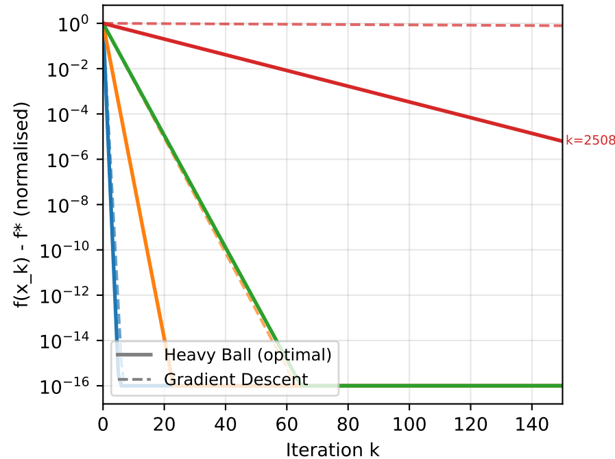
Heavy Ball vs GD for Various Kappas
