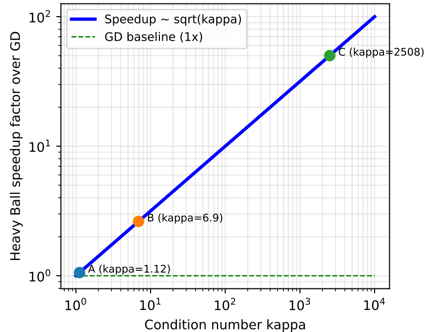
Speedup: Heavy Ball vs GD
