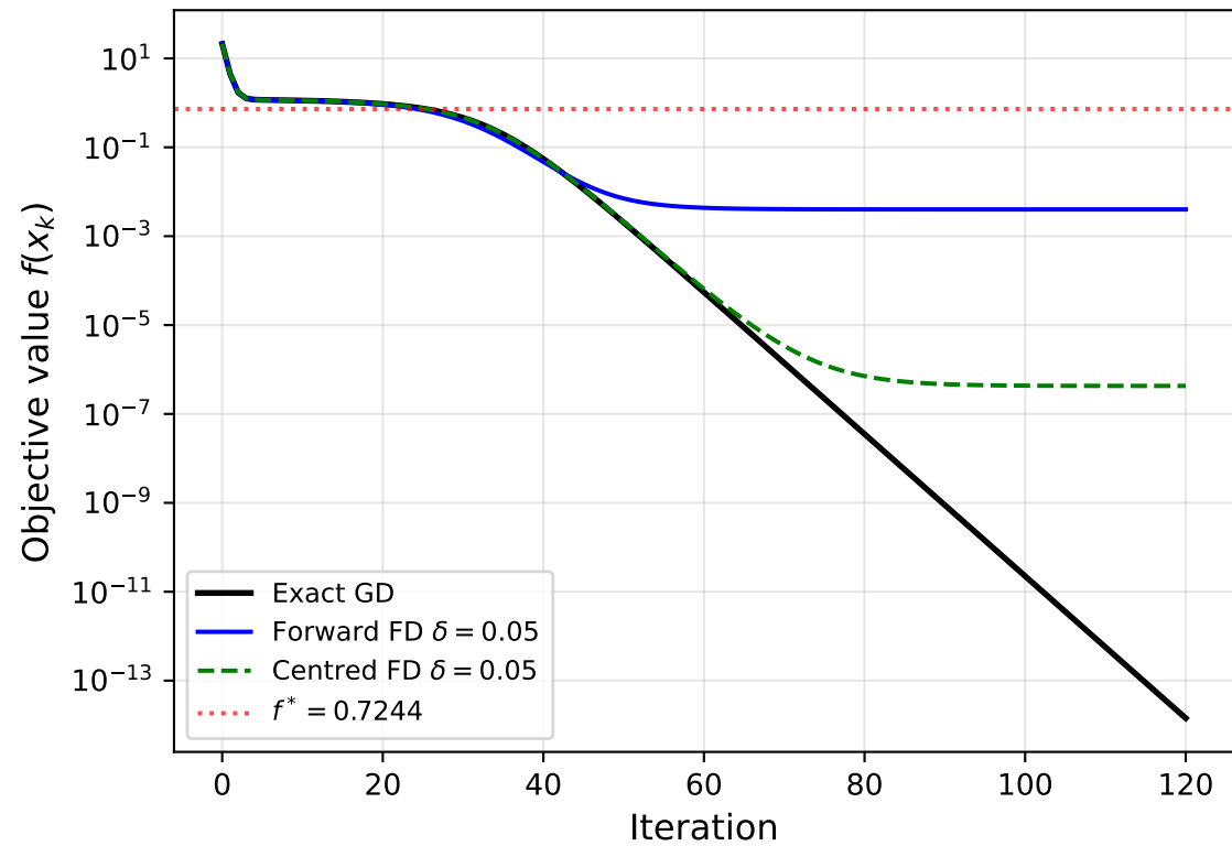
Forward vs Centred FD: \delta = 0.05 (near-optimal)
