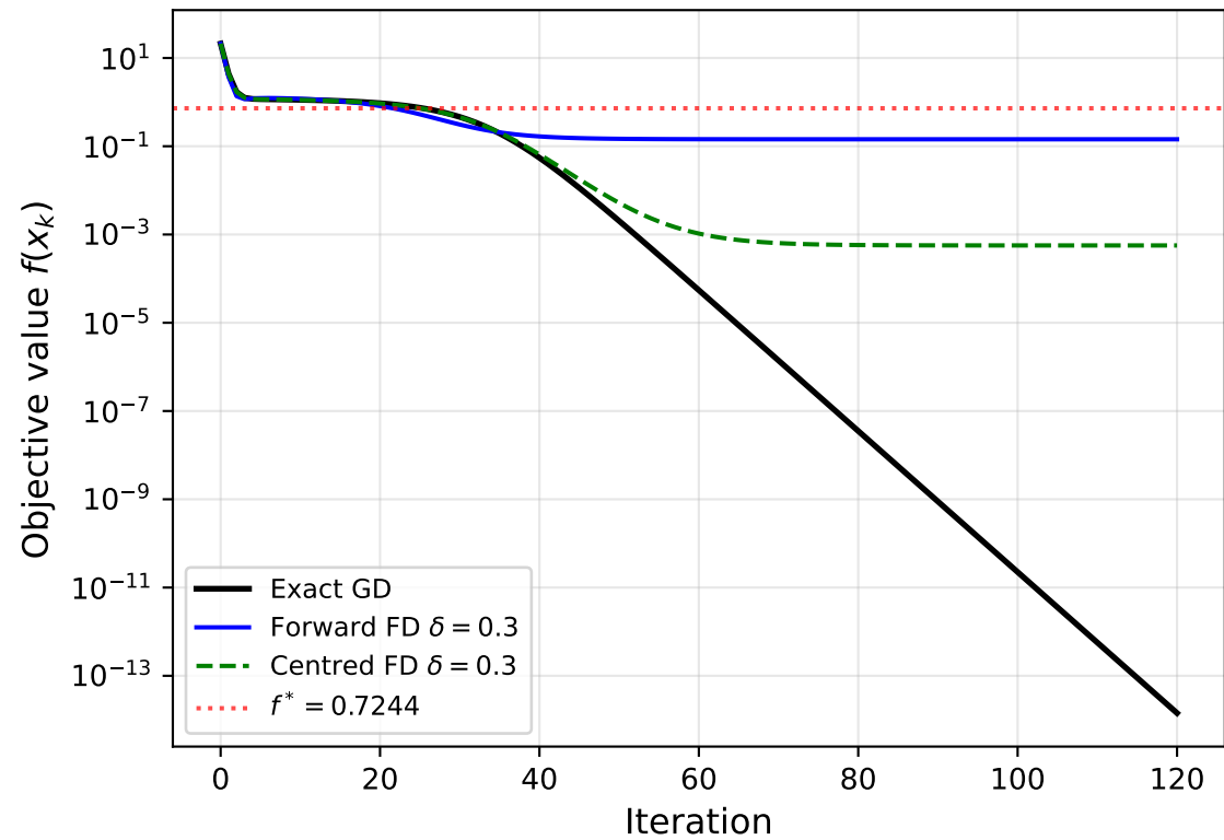
Forward vs Centred FD: \delta = 0.3 (moderate truncation)
