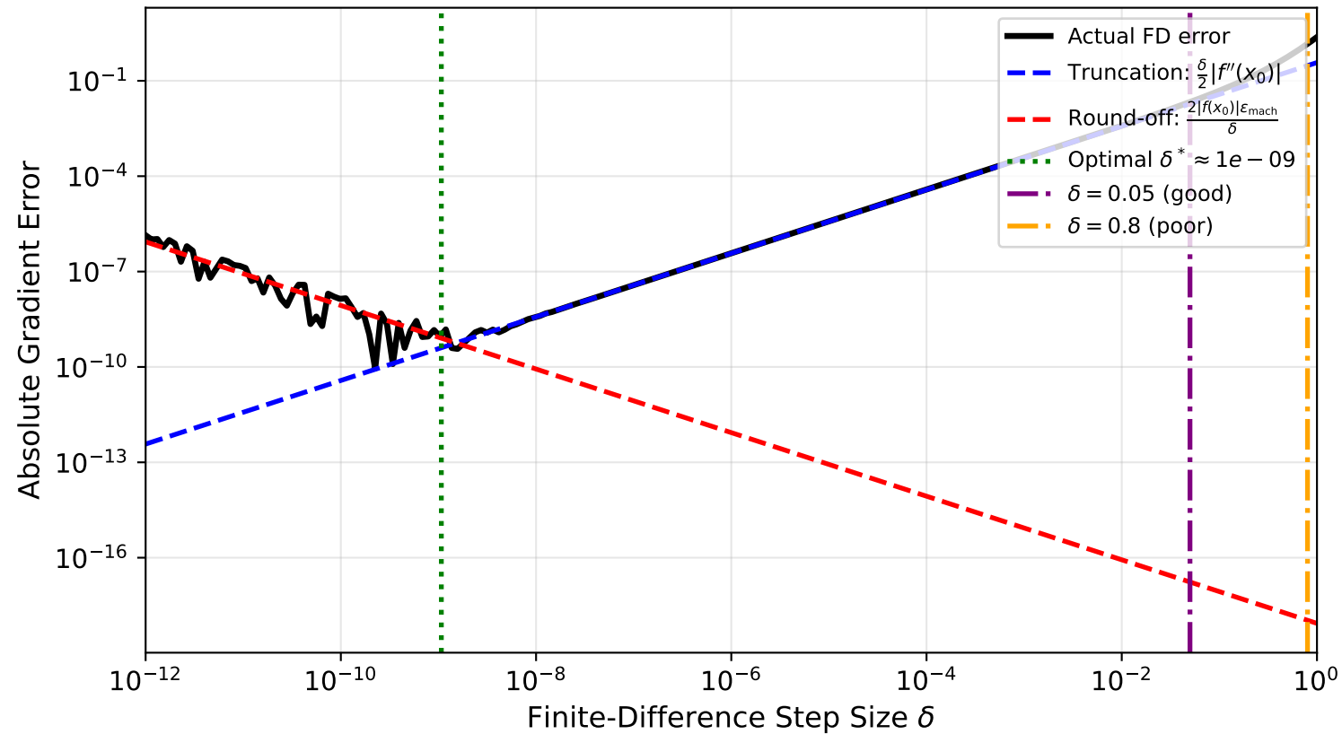
Q4: Finite-Difference Error vs. Step Size (g(x) = x^4 \text{ at } x_0 = 0.25)
