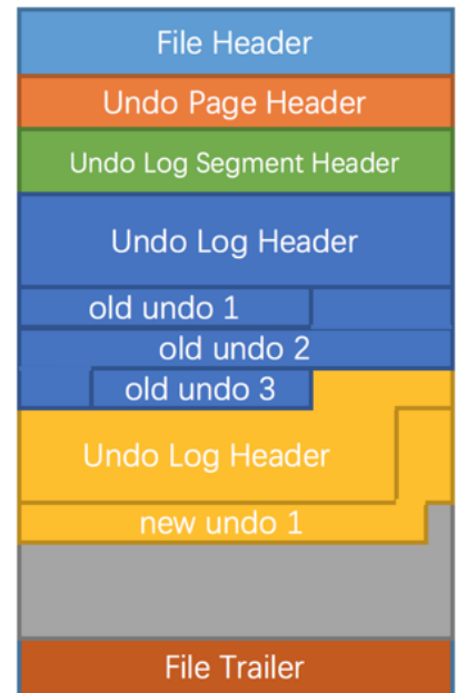
first undo page意图
