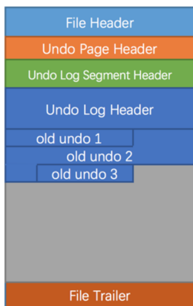
first undo page意图
