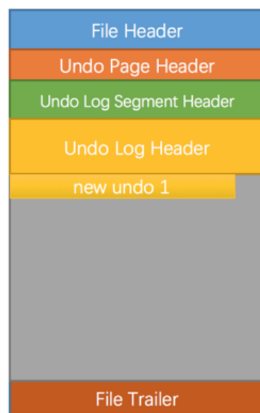
first undo page意图
