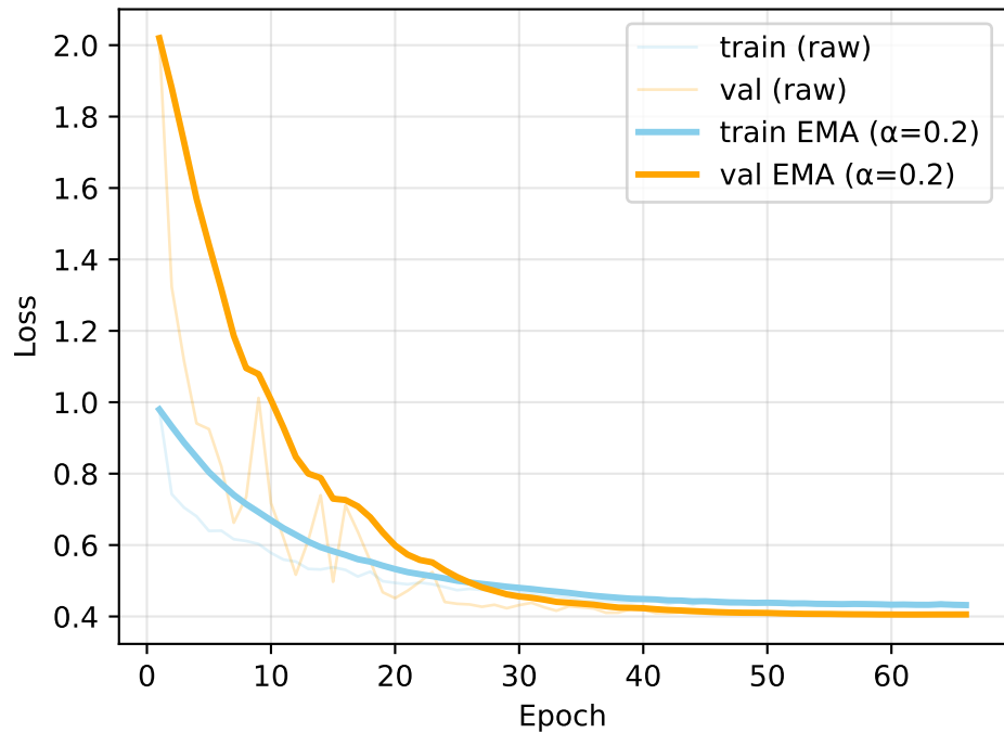
Loss (raw + EMA)
