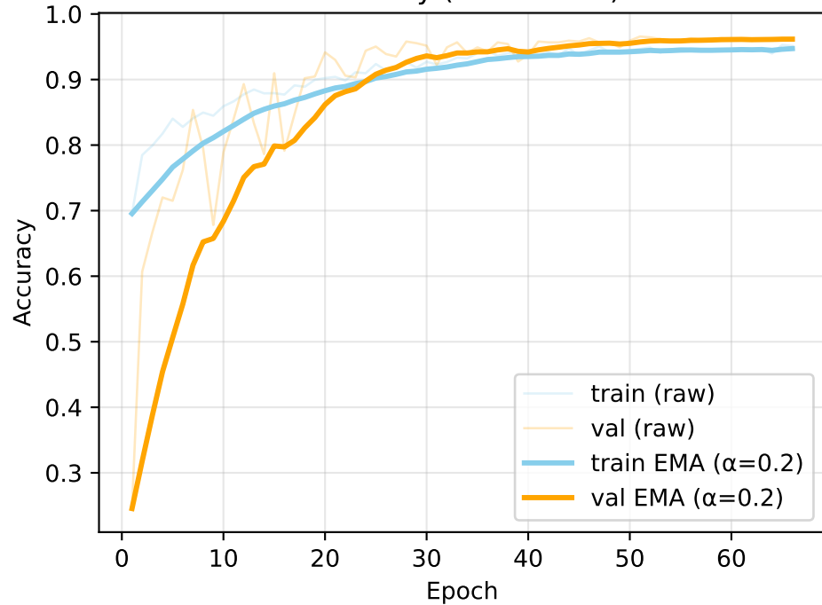
Accuracy (raw + EMA)
