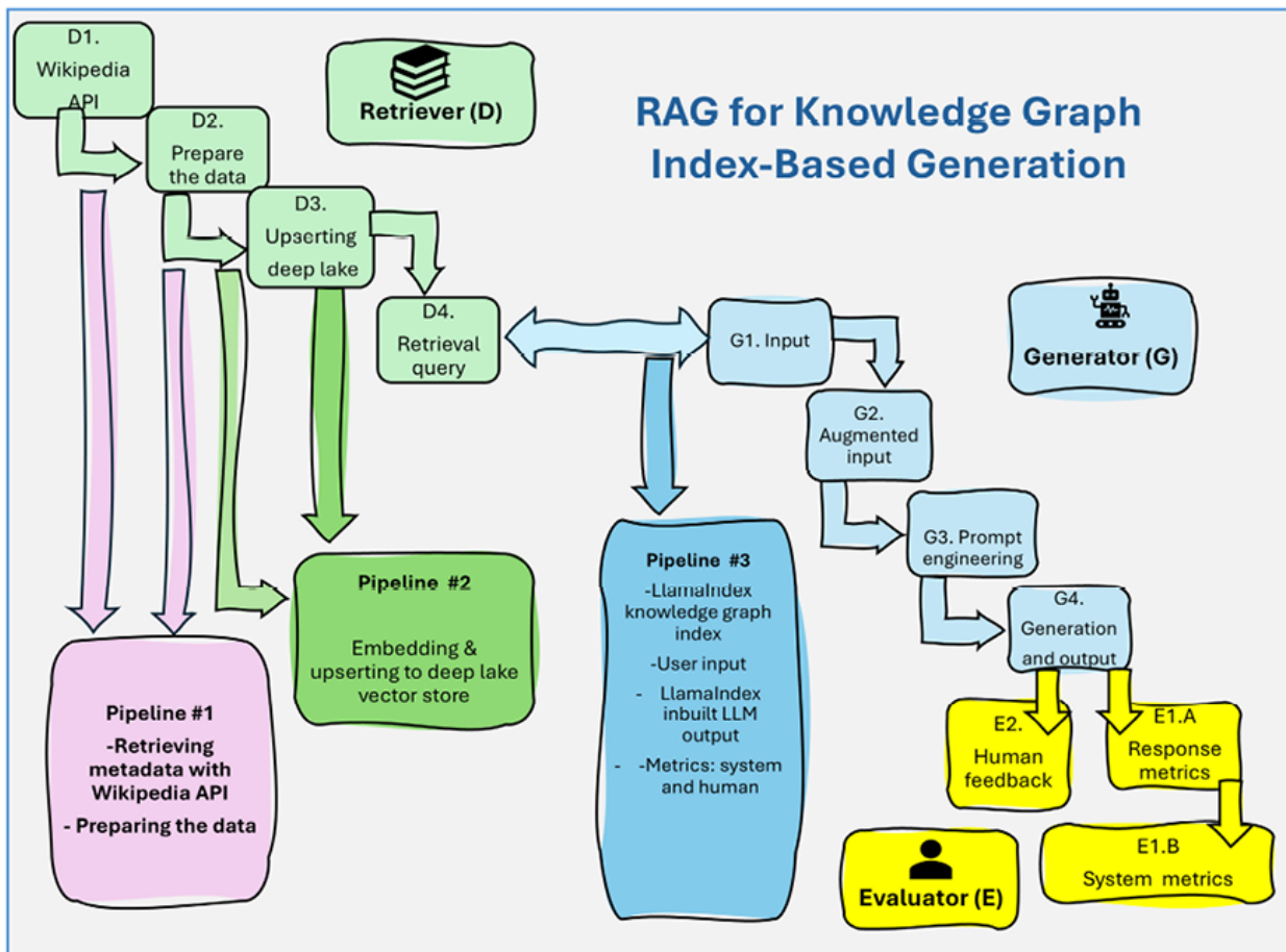
Figure 7.2: Knowledge graph ecosystem for index-based RAG
