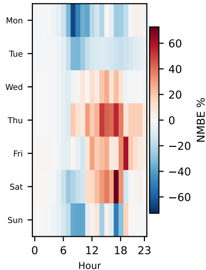
NEUTRAL (high CVRMSE) (Santos, Education)
