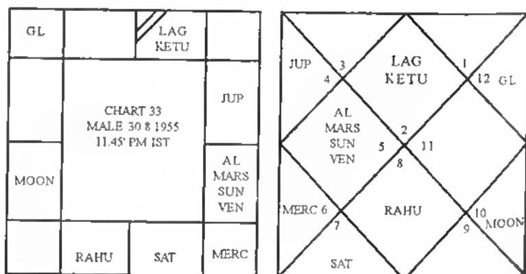
Chart 33. Male born on 30th August 1955 at 11.45" PM IST
