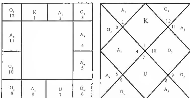
Fig 2.3: Schematic representaion of argala's on a hypothetical Karaka placed in Aries. The Argalas (A) and their obstructions (O) have been shown in suffix.
