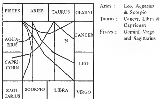
Fig. 2.2 Example of Rasi Dristi
