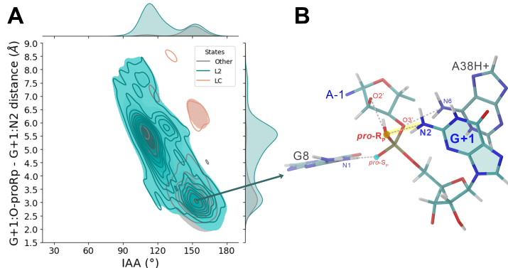
Figure 4: 2D distribution of the distances between protonated Opro-Rp phosphate oxygen and G+1:N2 against the Inline Attack Angle (IAA) in the protonated pro-Rp intermediate of the inline monoanionic scenario (A), together with a 3D view of the catalytic site in the high IAA region (B). The d_{OproRp-G+1:N2} is highlighted in yellow to emphasize the role of the 2-amino group of G+1 in the stabilization of the IAA flat junction.
