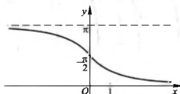
y = \operatorname{arccot} x
