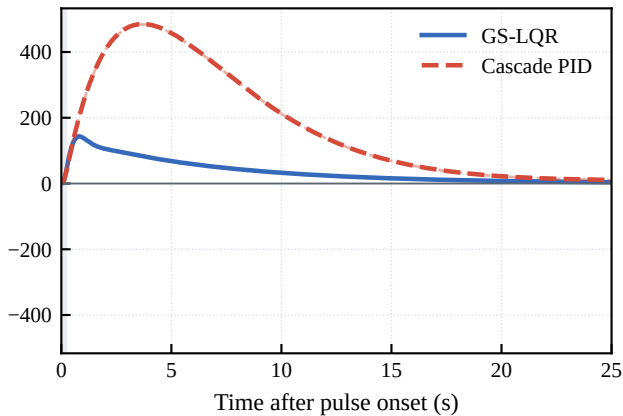
(a) +20 N, 0.20 s
