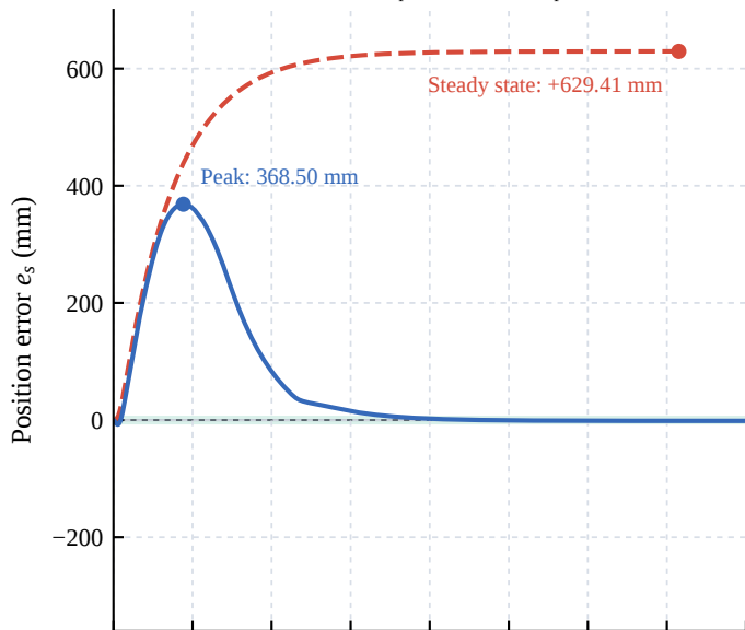
(a) Front payload: m_p = 1.0 kg, \Delta y_p = +0.10 m
