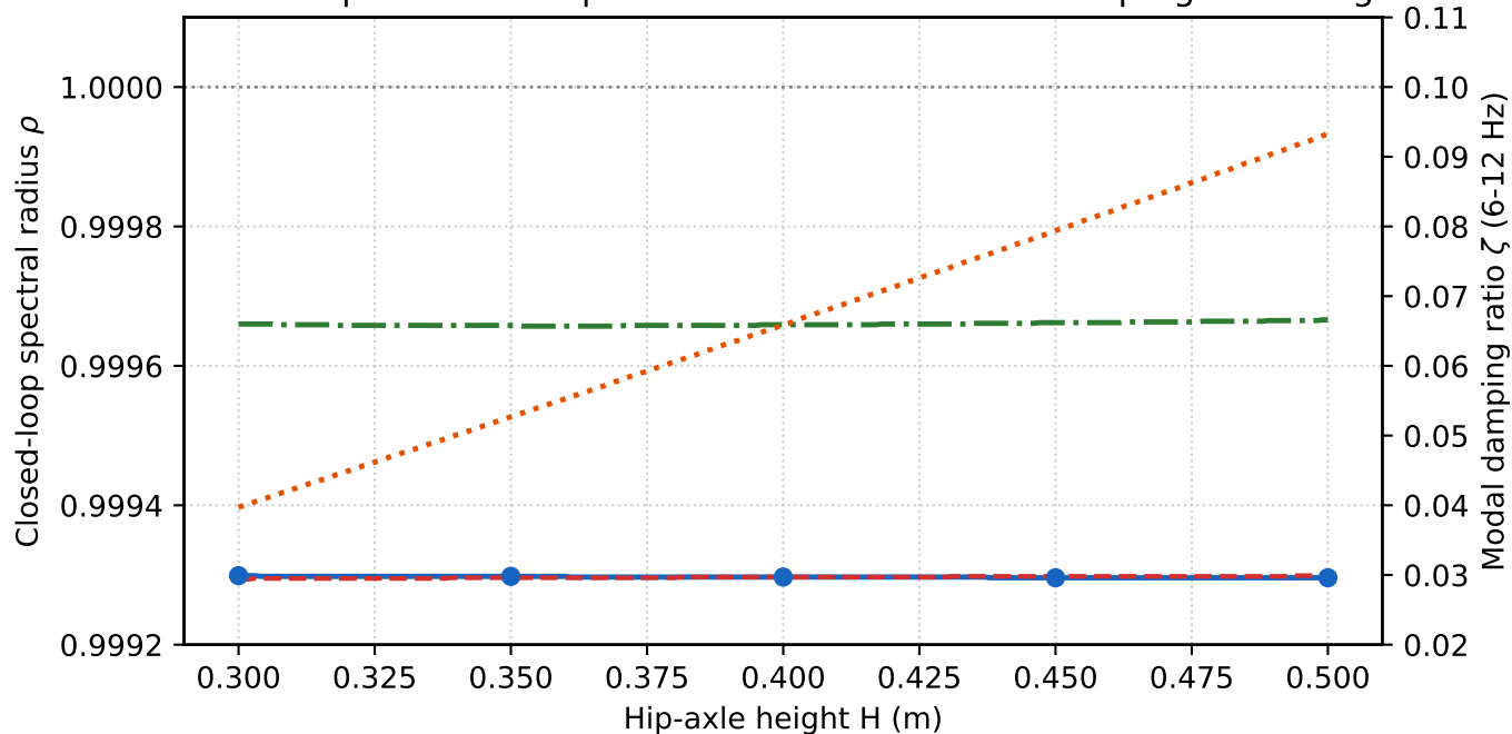
Closed-loop multi-rate spectral radius and modal damping over height
