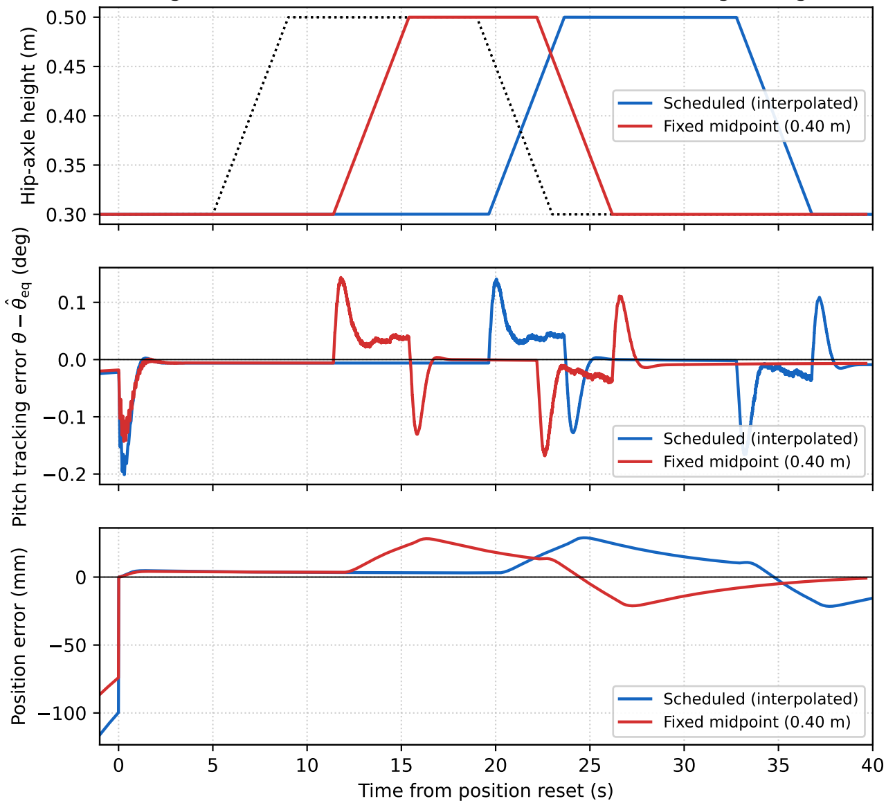
Height transition 0.30 -> 0.50 -> 0.30 m (dotted: target height)
