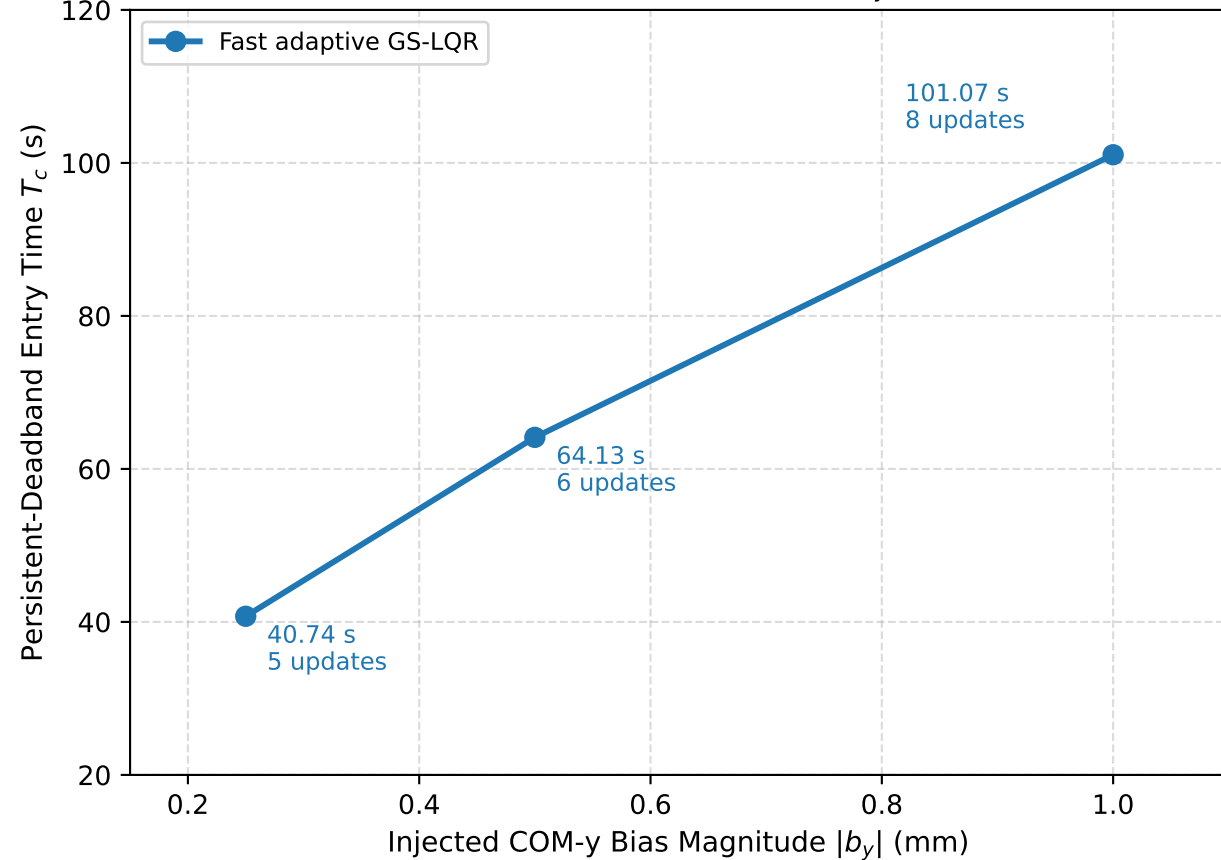
(b) Adaptive Convergence: |b_y| vs. T_c
