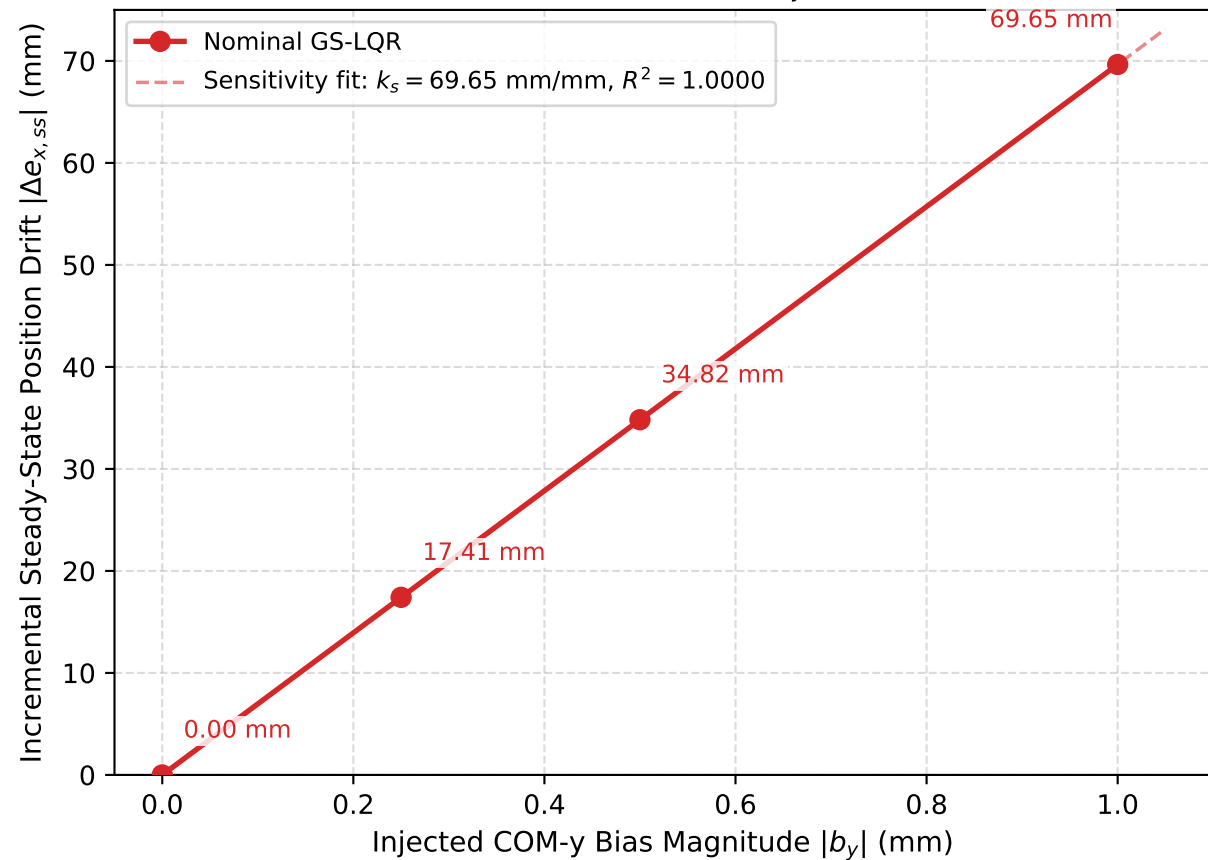
(a) Nominal Sensitivity: |b_y| vs. |\Delta e_{x,ss}|
