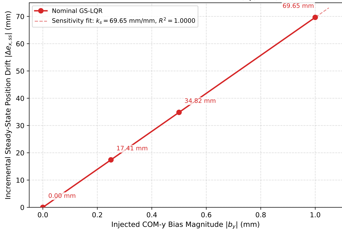
Nominal Model-Mismatch Sensitivity: |b_y| vs. |\Delta e_{x,ss}|
