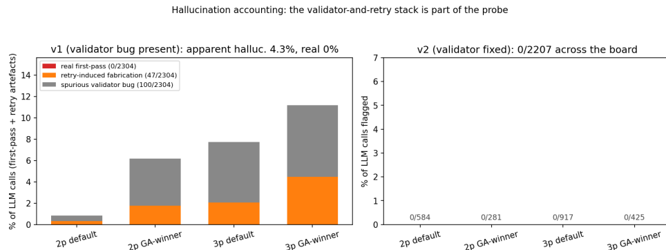
Figure 16: A faulty validator pulls the model toward fabrication. Per-call validation outcomes for v1 (buggy validator) and v2 (fixed). Categories: real first-pass fabrication, retry-induced fabrication (a correct first output that the buggy validator flagged, then “corrected” to a wrong answer), and spurious flags (correct outputs falsely flagged). v1 over 2,304 calls: 0 real, 47 retry-induced, 100 spurious; v2 drives all three to zero over 2,207 calls. Second-order lesson: validating against a wrong ground truth is worse than not validating.
