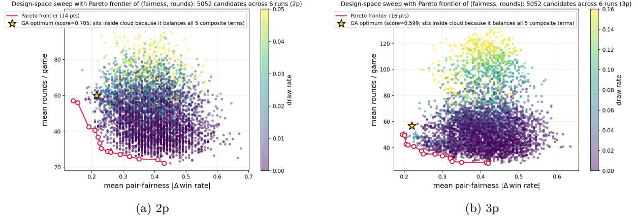
Figure 13: The (fairness, rounds) trade-off surface and its Pareto frontier. Each marker is one of 5,052 candidates from all six search runs (random + GA + four ablations); colour encodes draw rate, and the crimson line is the 2D Pareto frontier (both axes minimised). The gold star is the combined-objective GA optimum; it sits inside the cloud because the composite weights five terms, not two, so its optimum lies on the 5D Pareto surface of which this is a projection. The 2p and 3p clouds have visibly different shapes, which is what makes the cross-evaluation finding (Table 2) a property of the design space, not seed noise.
