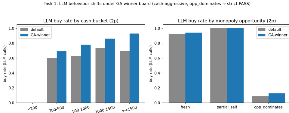
Figure 15: LLM buy-rate slices, default vs. GA-2p winner. (a) By cash bucket: buy rate rises monotonically with available cash (the empty < 200 bucket reflects the affordability pre-filter); on the GA winner the LLM commits its hoard more aggressively at \geq 1500 ( \sim 0.93 vs. \sim 0.70 ). (b) By monopoly situation: \sim 1.00 when it already partly owns the group ( partial_self ), \sim 0.94 on a fresh group, and \sim 0.13 when the opponent dominates it ( opp_dominates ). The probe responds rationally, not as a uniform-random oracle, and near-identically on both boards.
