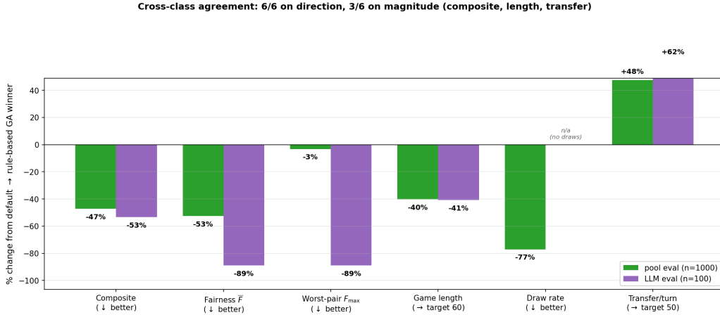
Figure 4: Both evaluator classes agree on direction for all 6 metrics (rule-based GA winner vs. default, 2-player). Per-metric % change under the 30-strategy pool (green, n=1000 ) and all-LLM seats (purple, n=100 ). Magnitudes match closely on composite ( -47\% / -53\% ), length ( -40\% / -41\% ), and transfer per player-turn ( +48\% / +62\% ); the two fairness terms agree in direction but diverge in magnitude (smaller LLM tail at n=100 ). Draw rate is in the panel footer because LLM seats produce no draws on either board.
