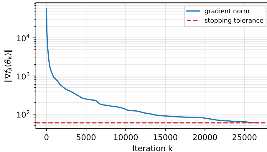
Gradient norm (log y-axis)
