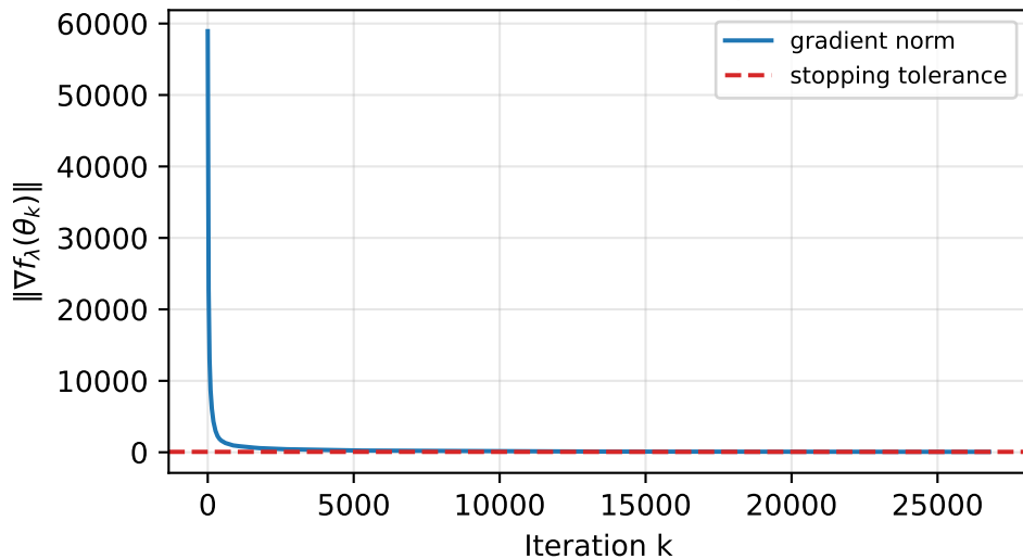
Gradient norm (linear y-axis)
