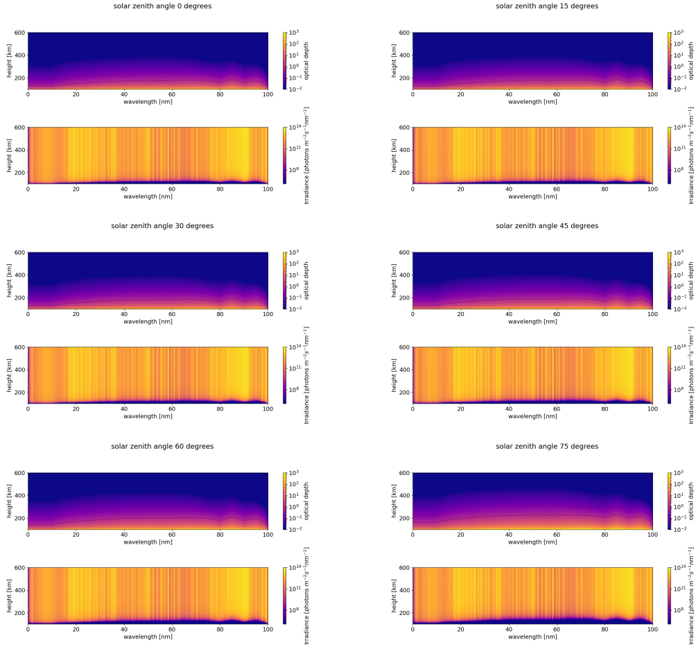
Figure 3: Optical depth and EUV photon fluxes for different angles of incidence.
