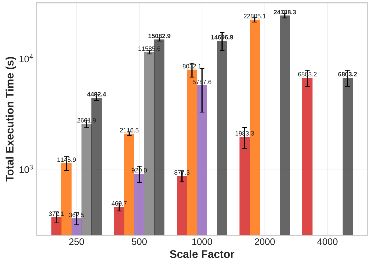
Total Execution Time by Scale Factor
