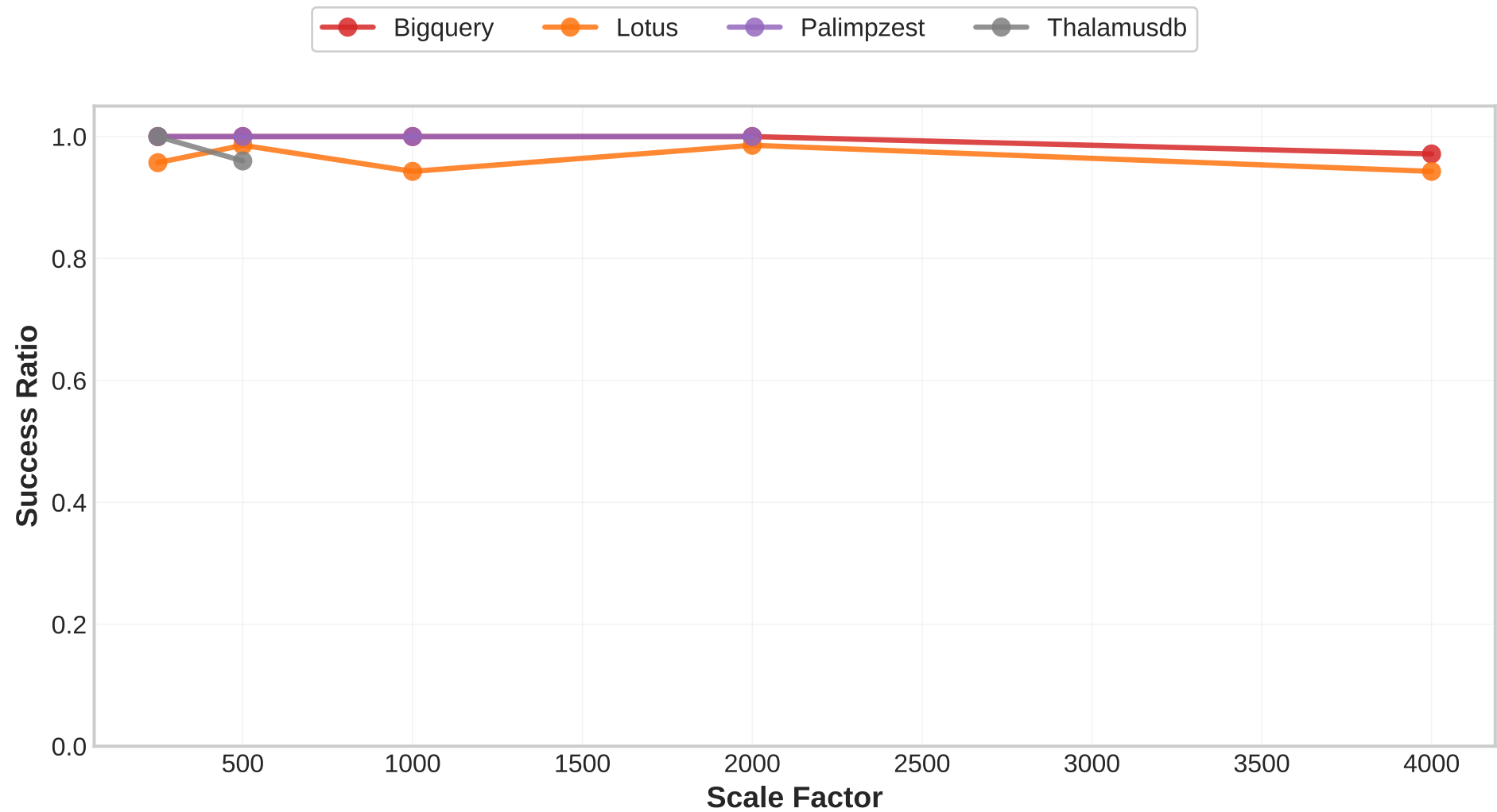
ECOMM: Success Ratio by Scale Factor
