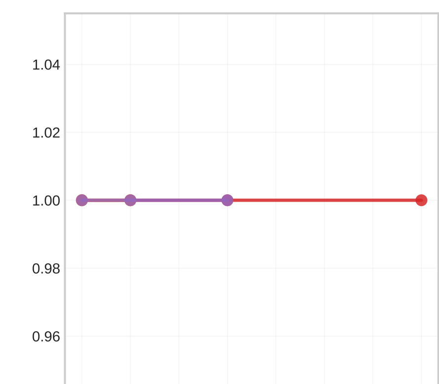
F1-Score / Accuracy
