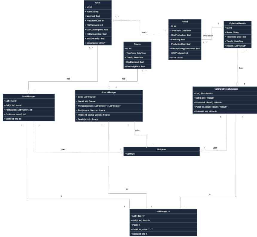
Figure 4.1: HeatItOn Abstract Class UML Diagram
