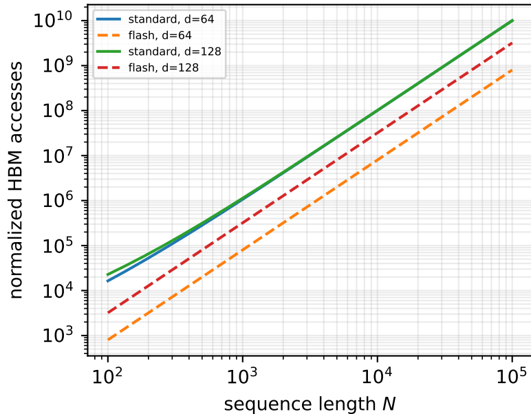
HBM-access scaling at 100 KiB SRAM
