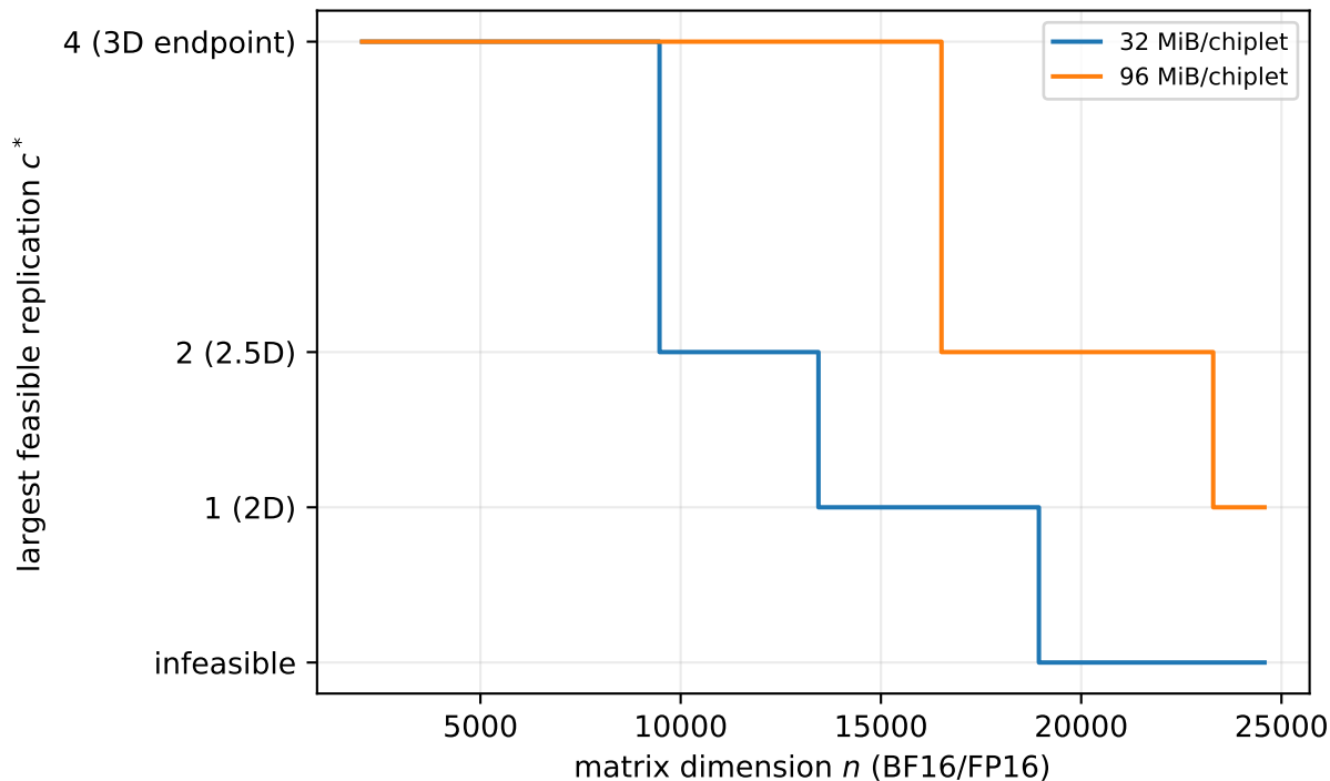
Certified 2.5D GEMM memory-replication phase map, P = 64
