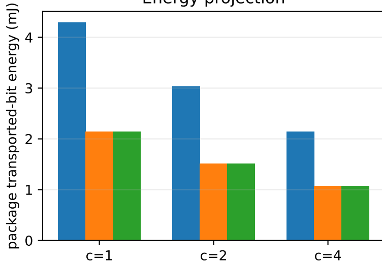
Energy projection
