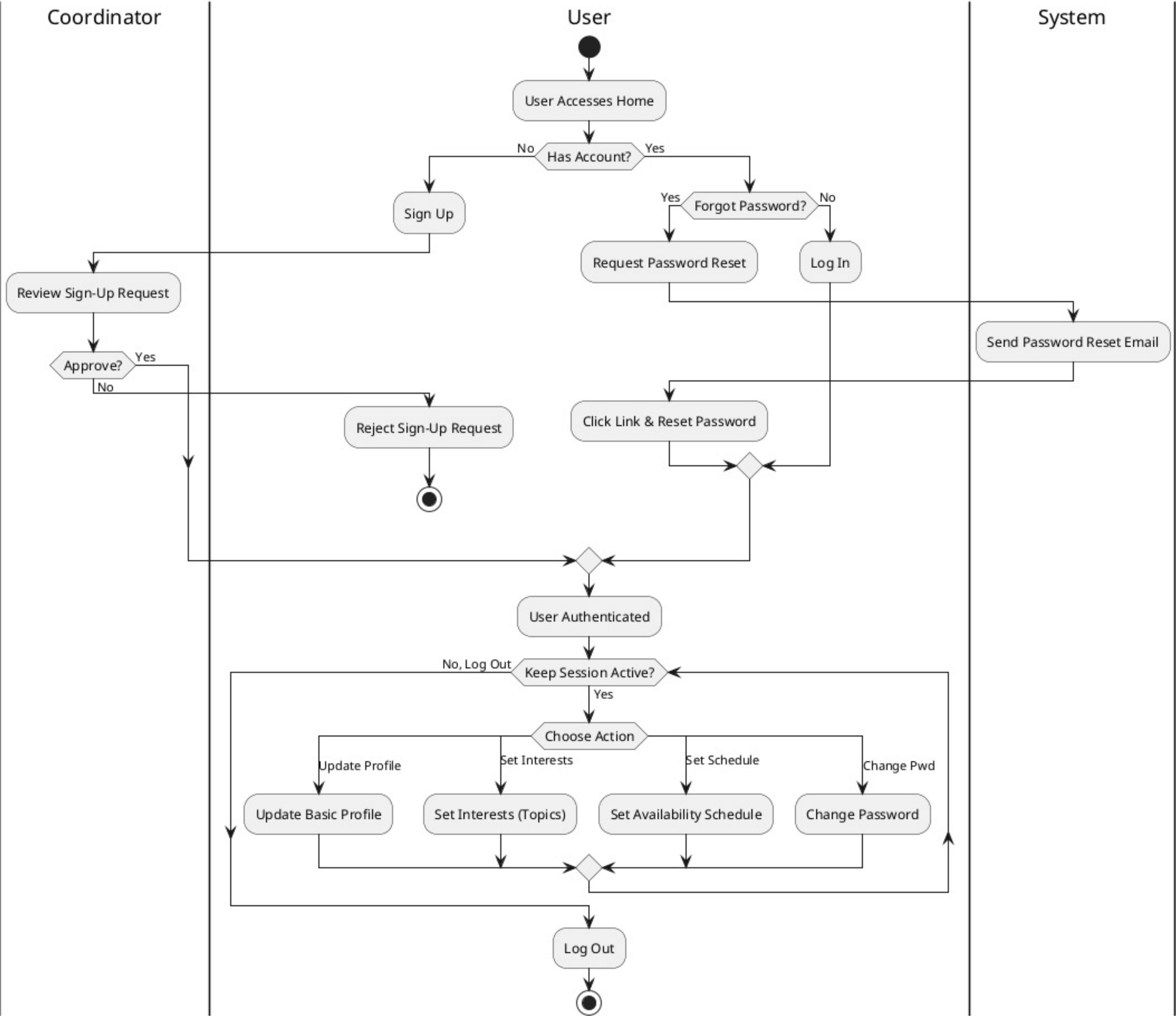
Account Management Activity Diagram
