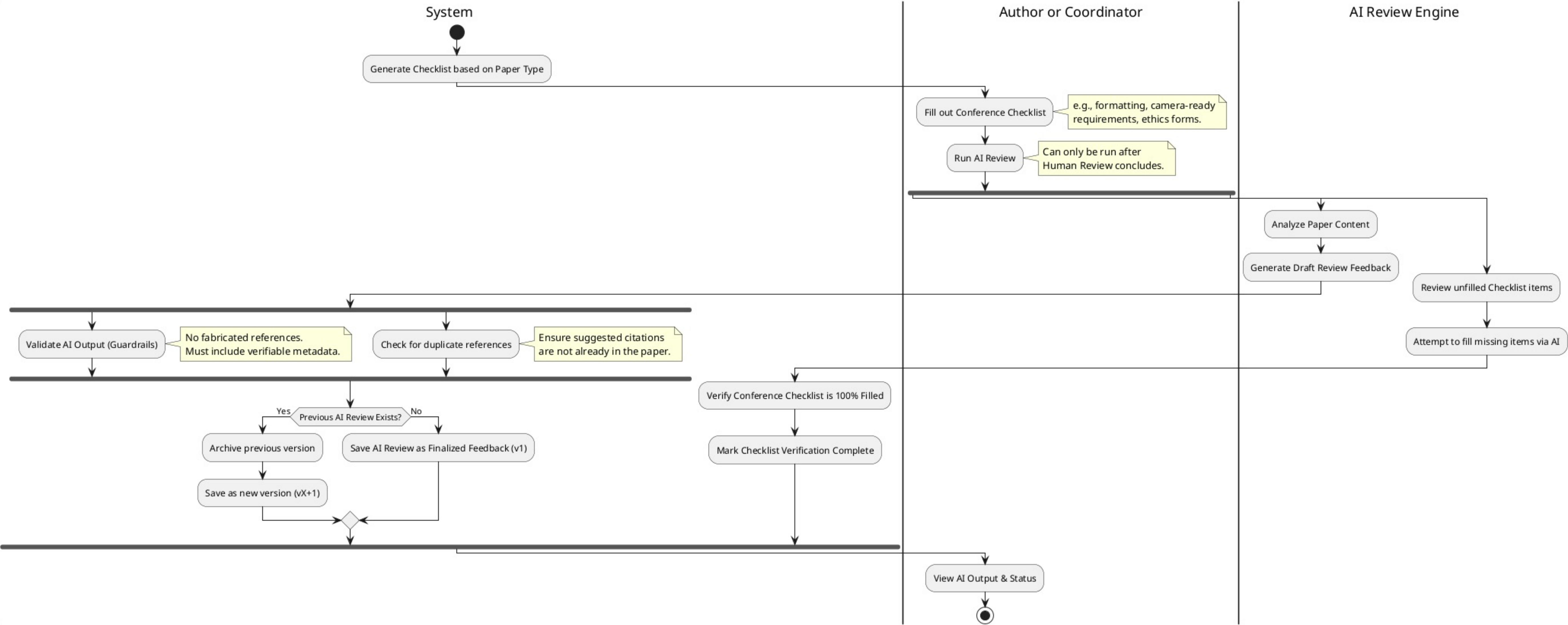
Post-Review Phase Activity Diagram
