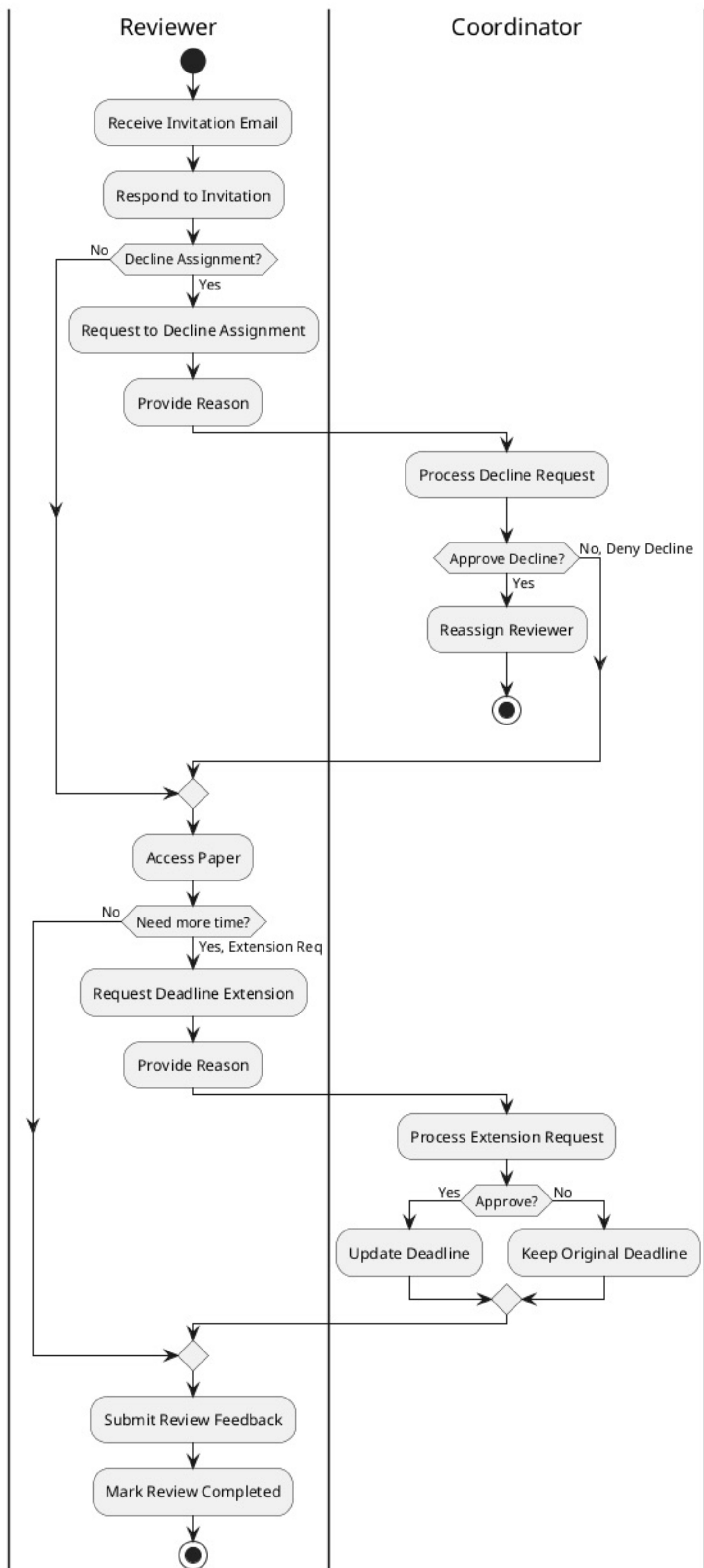
Reviewer Response Activity Diagram
