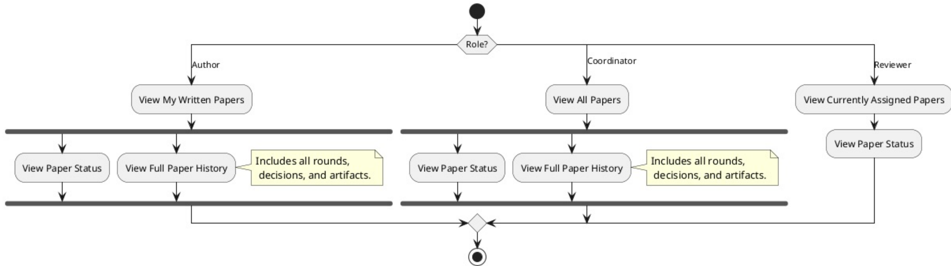
History Viewing Activity Diagram
