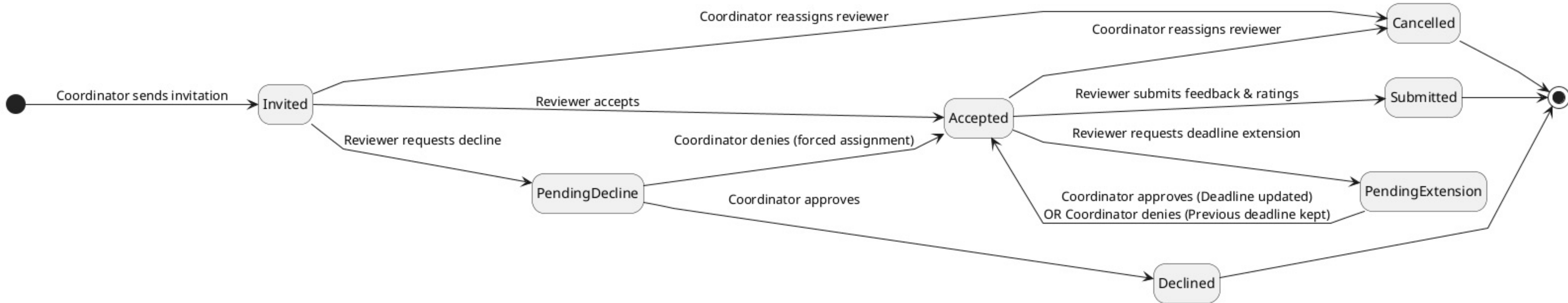
Reviewer Assignment State Diagram
