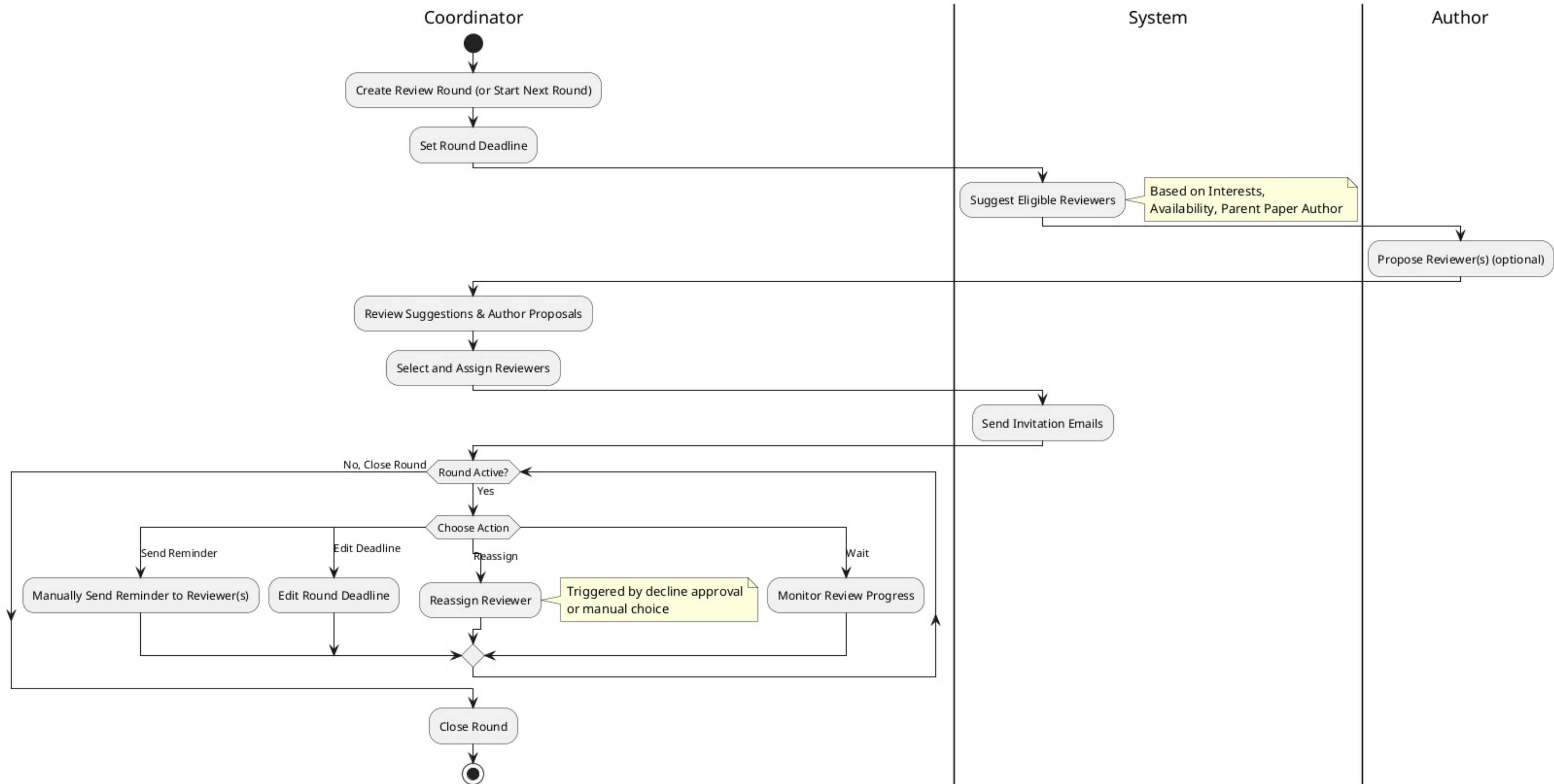
Round Management Activity Diagram
