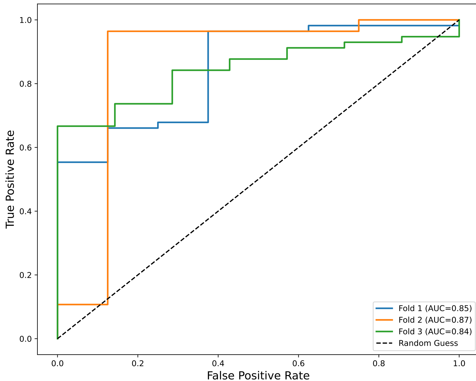
ROC Curves of All Folds
