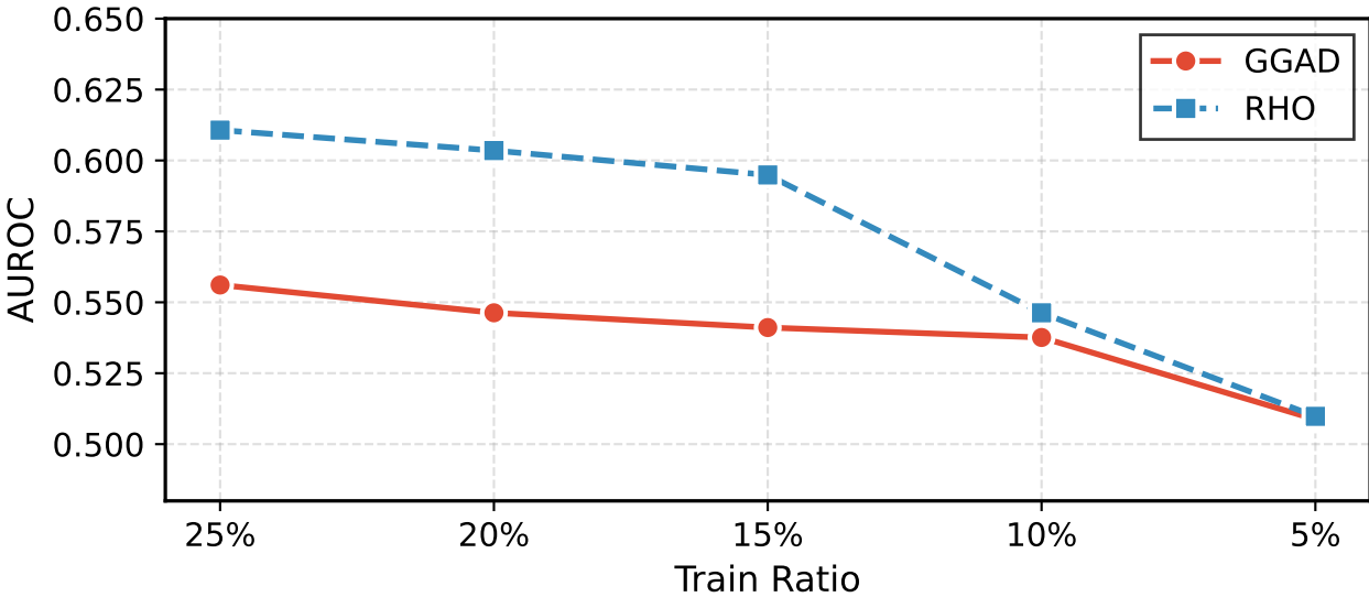
(a) AUROC
