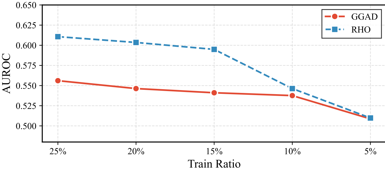
(a) AUROC
