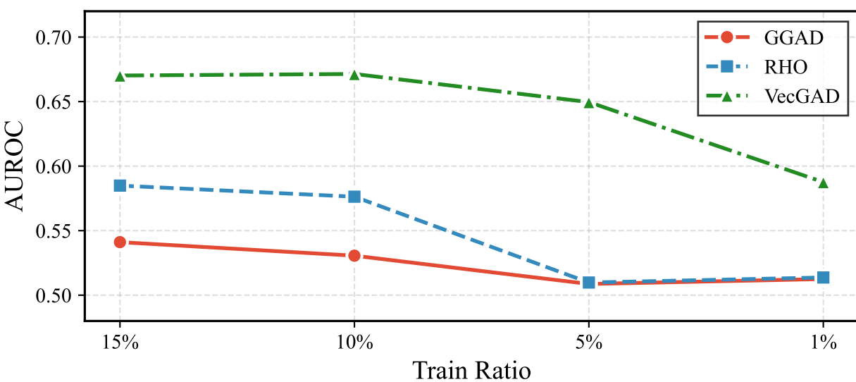
(a) AUROC
