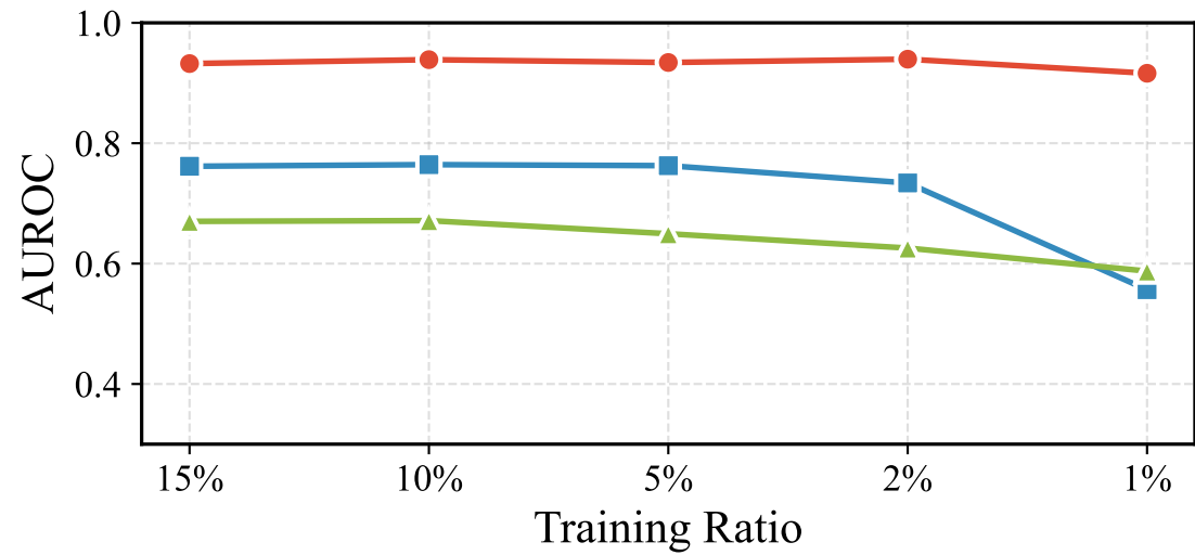
(a) AUROC
