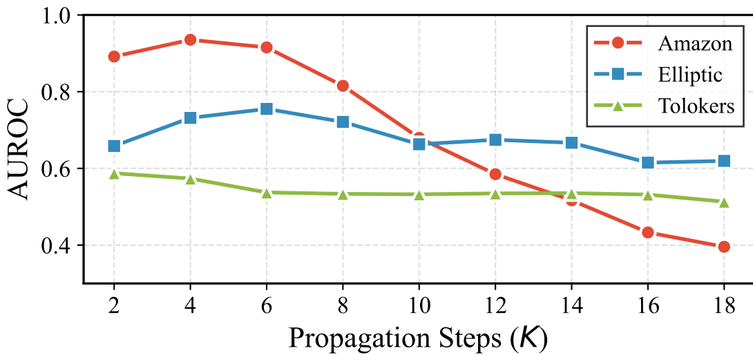
(a) AUROC
