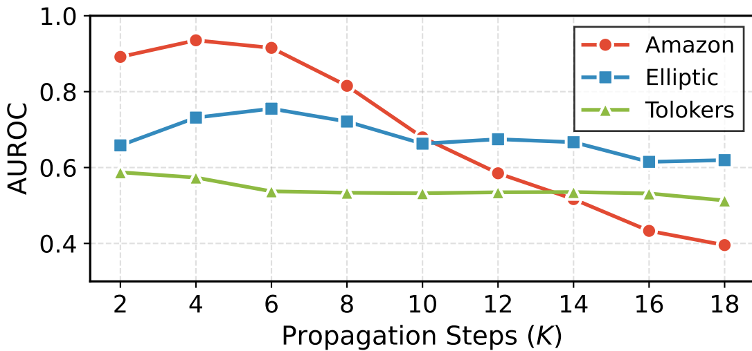
(a) AUROC
