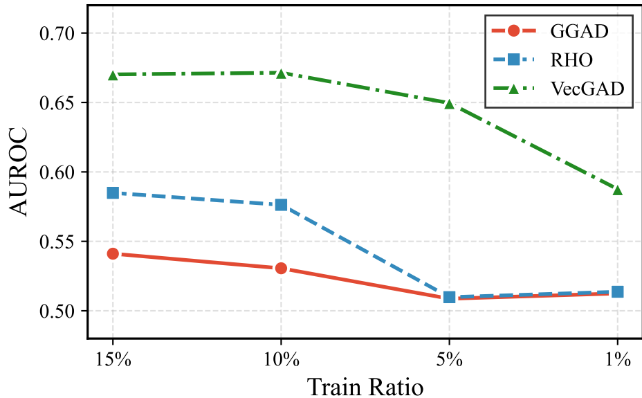
(a) AUROC
