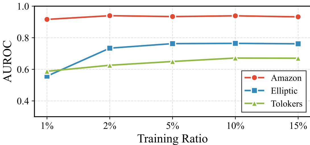
(a) AUROC
