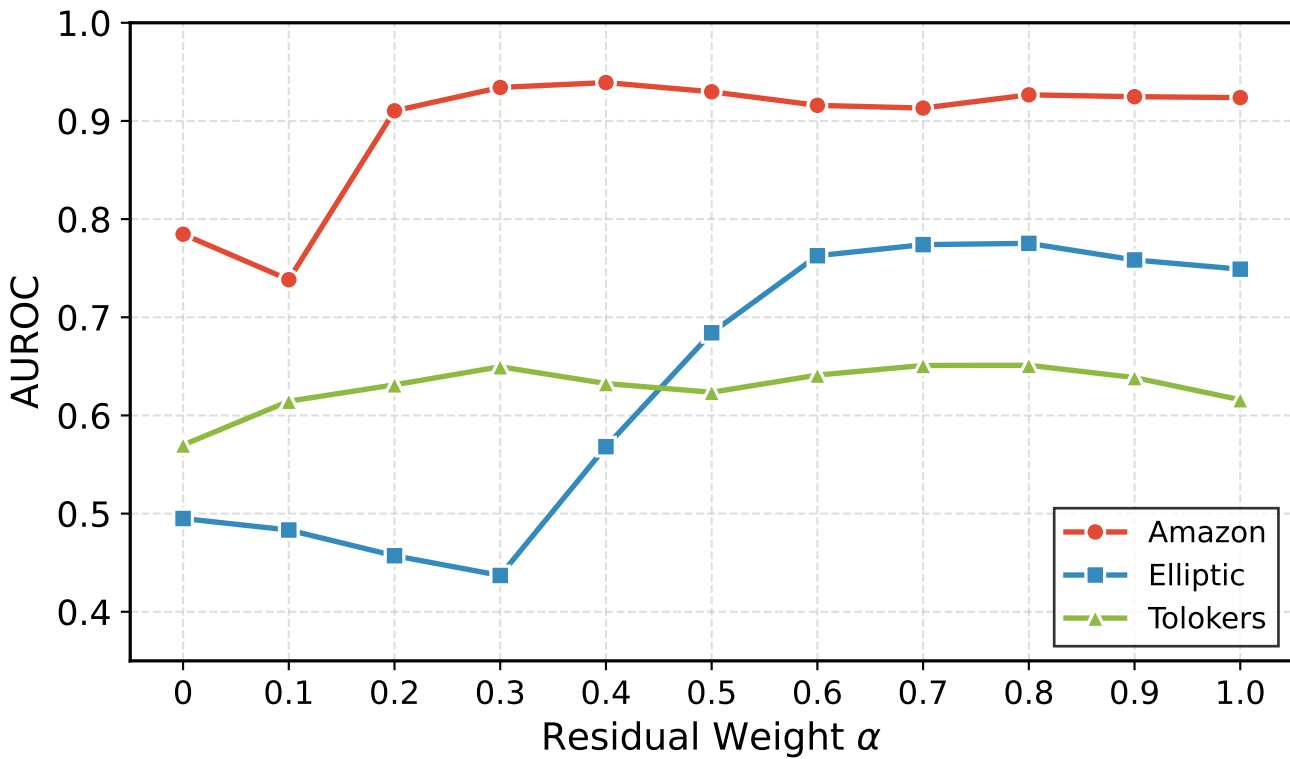
(a) AUROC
