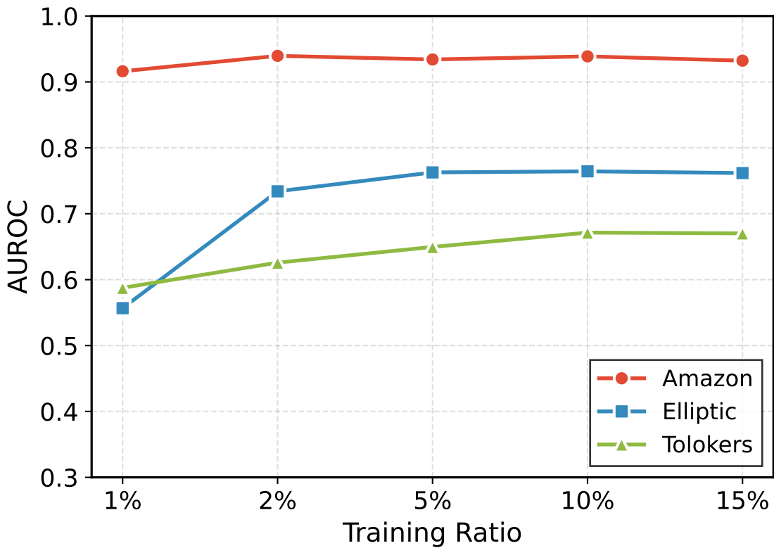
(a) AUROC
