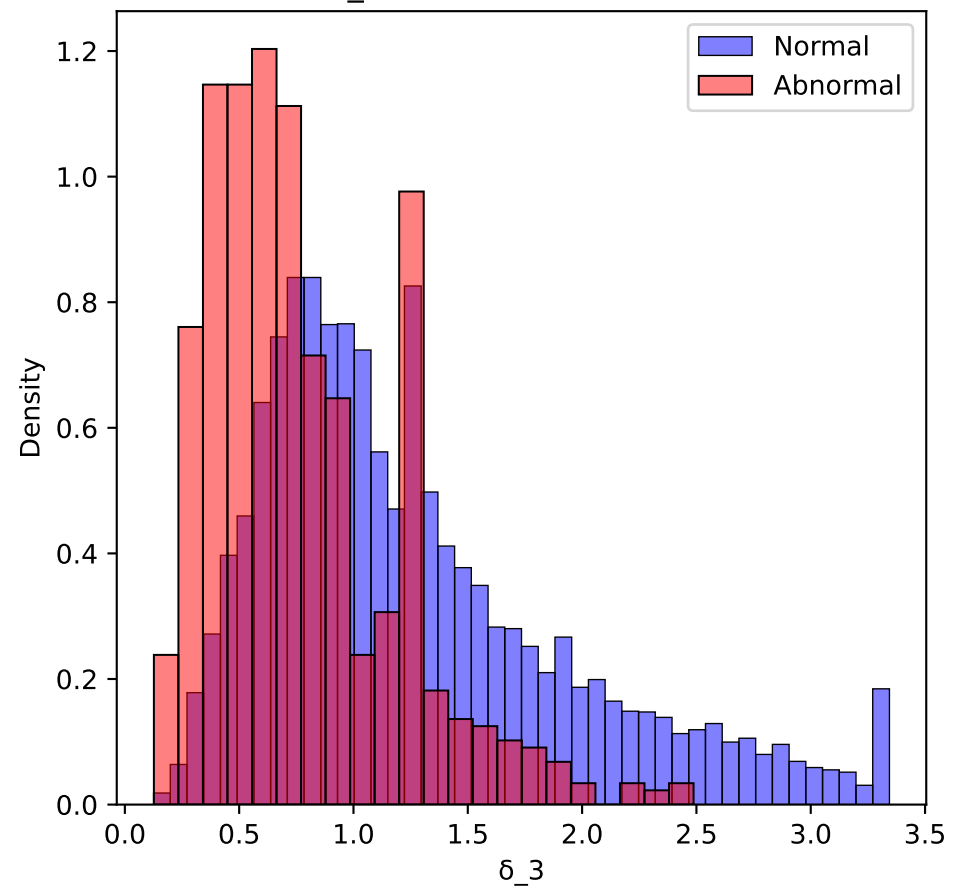
\delta_3 Distribution ( \alpha=0.2 )
