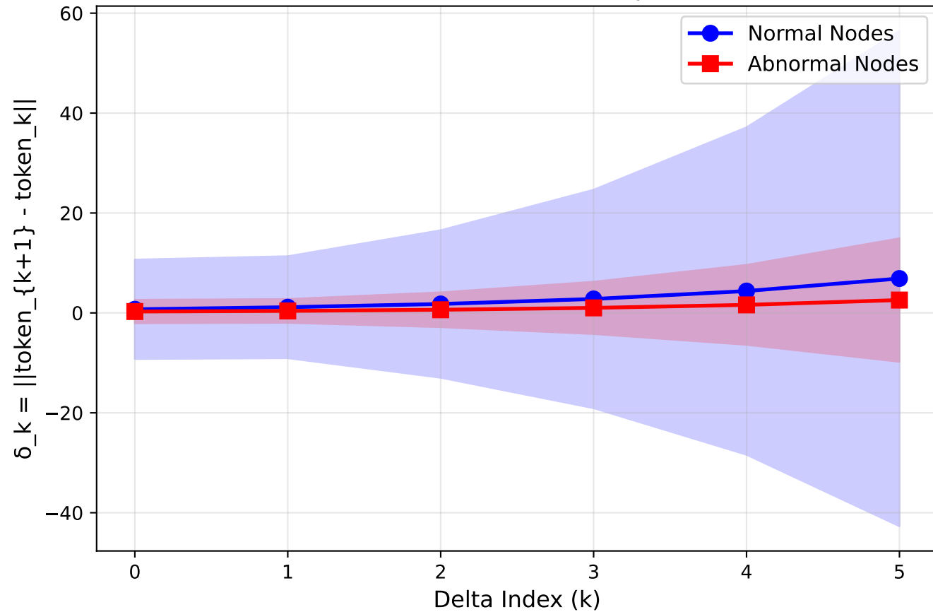
ISP Delta Curves - elliptic
