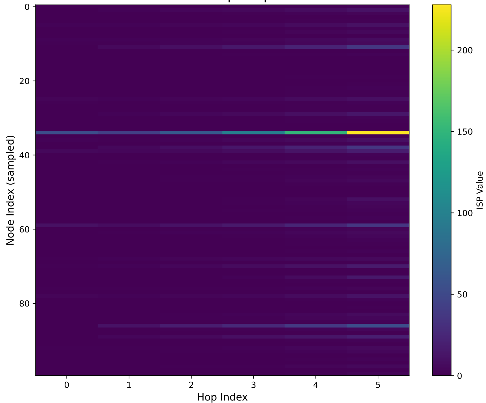
ISP Heatmap - elliptic
