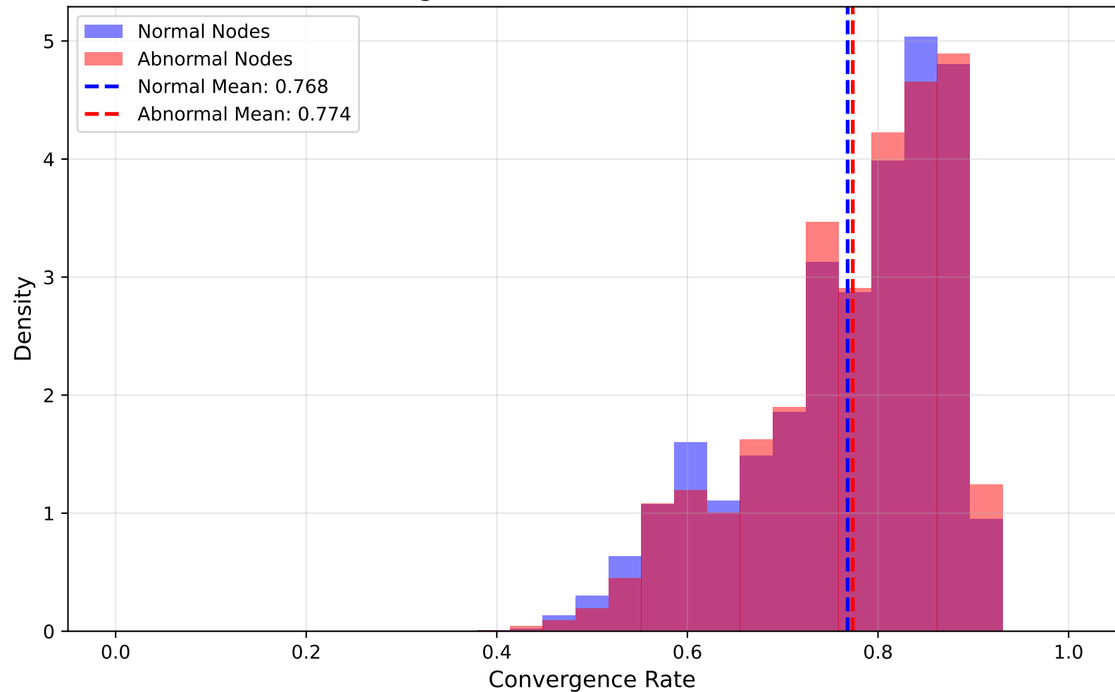
Convergence Rate Distribution - tolokers
