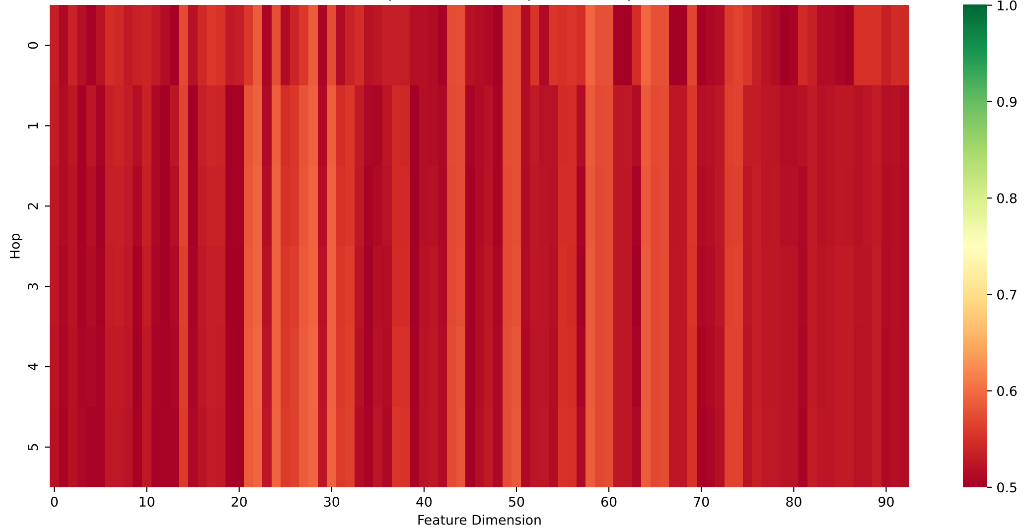
Feature Importance Heatmap (AUC) - elliptic
