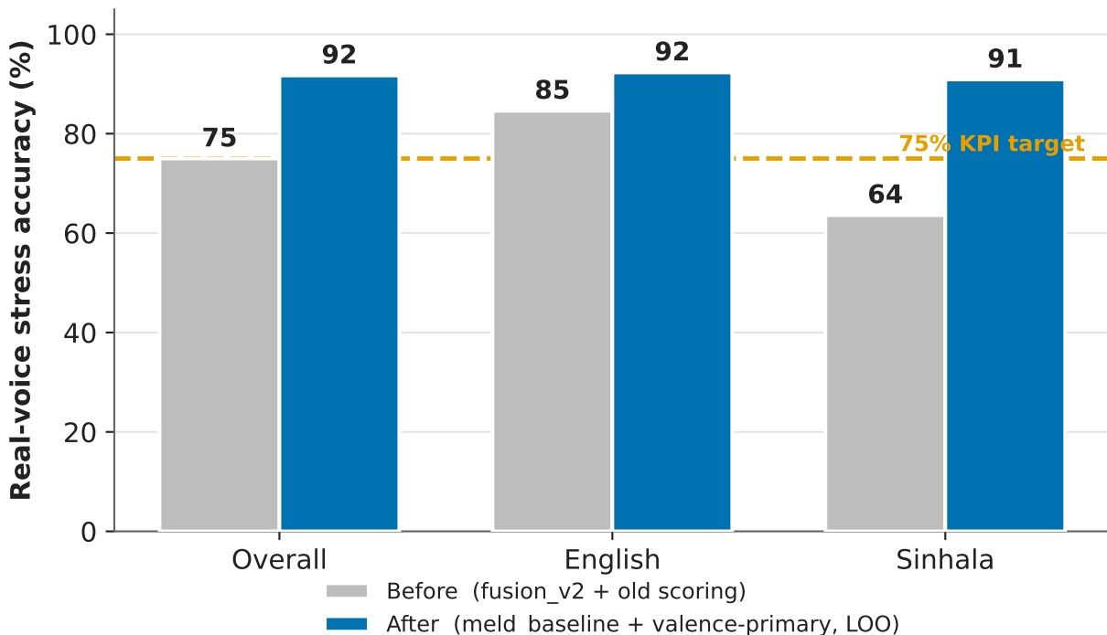
Component D — real-voice accuracy before vs after Phase 1 (valence-primary scoring + evidence-based model selection)
