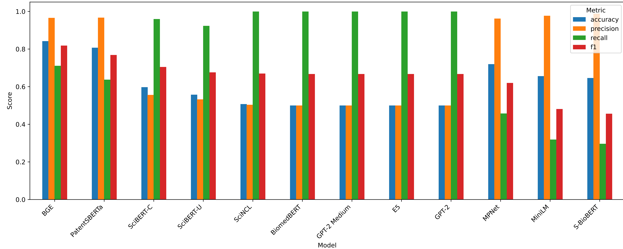
Model Performance Metrics — Coleoptera
