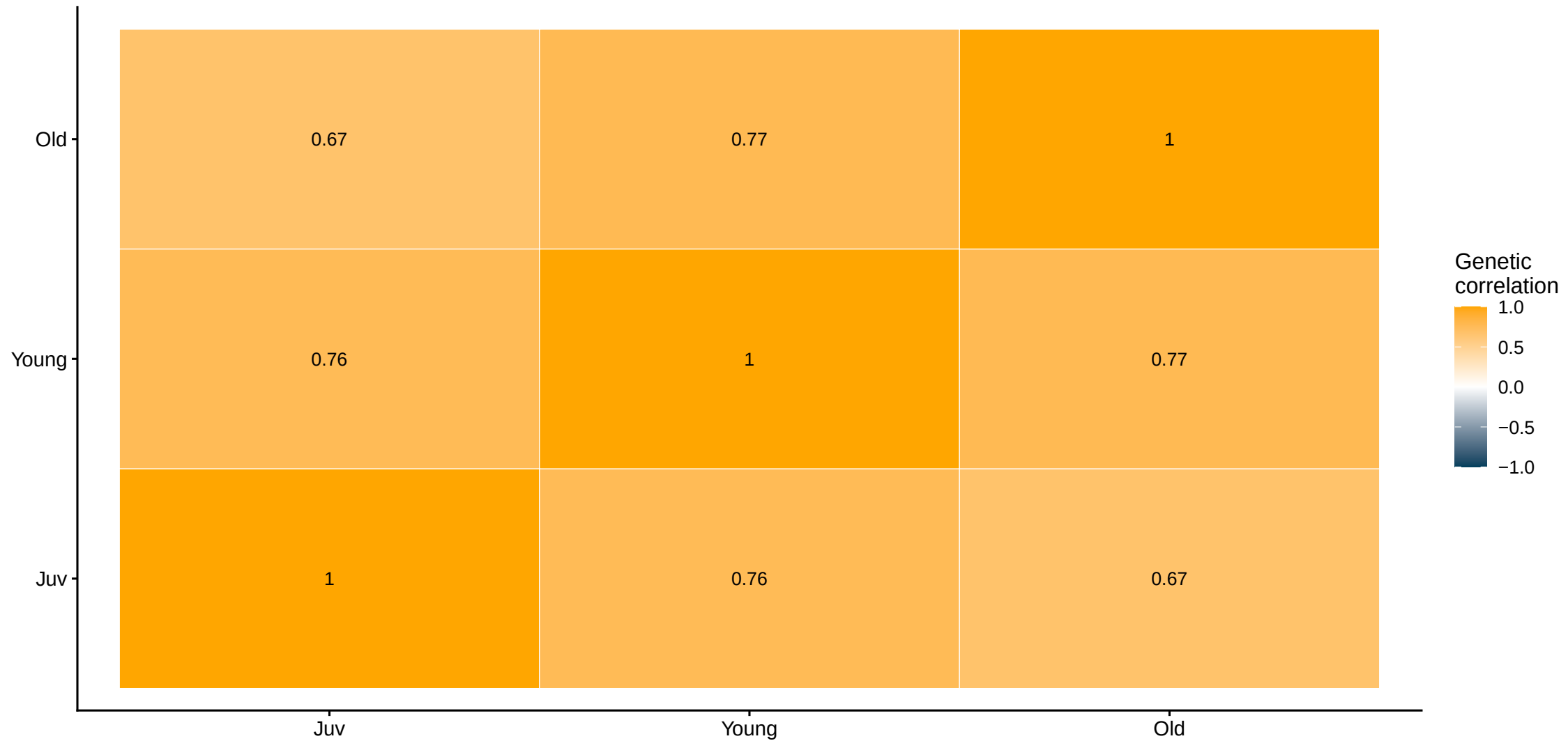
Genetic correlations across age classes (model_CS)
