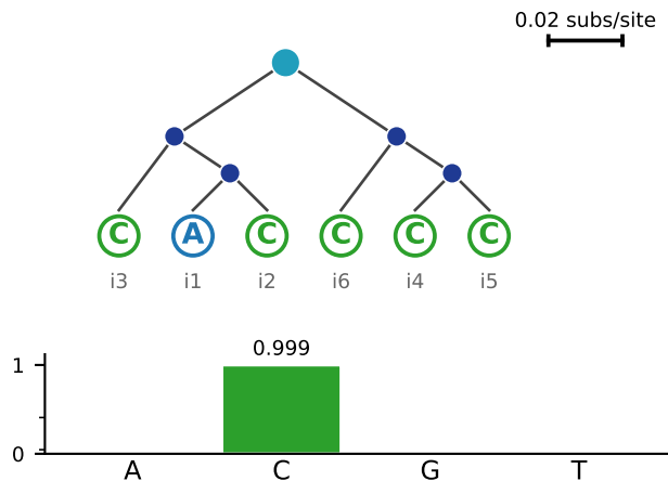
(b) Near-fixed derived ( i = 5 )
