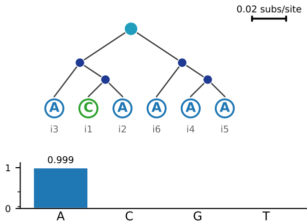
(a) Singleton derived ( i = 1 )
