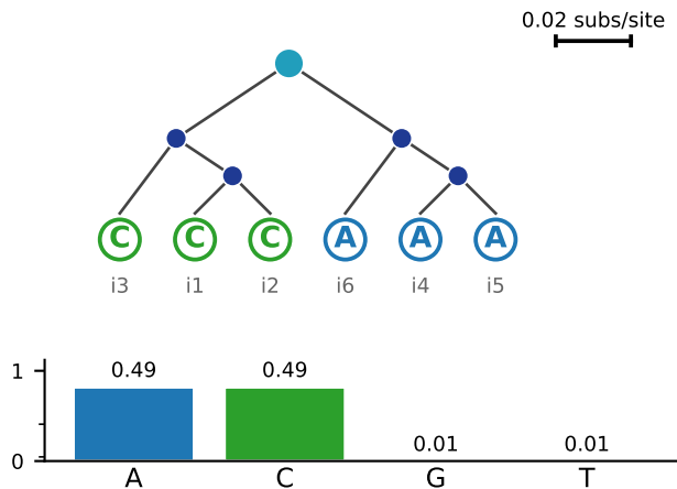
(c) Clade-aligned split ( i = 3 )
