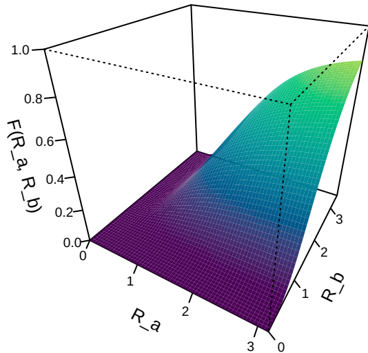
Joint CDF
