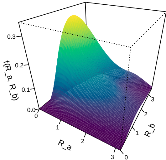
Joint density
