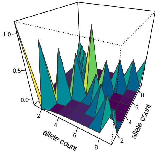
Kingman
