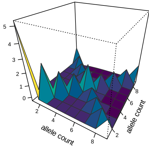
Beta
