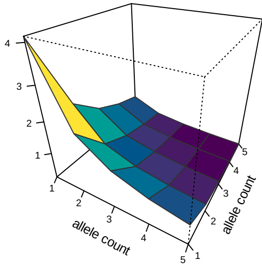
Near-independent ( r = 10 )
