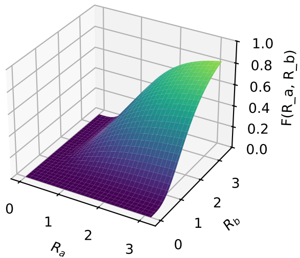
Joint CDF
