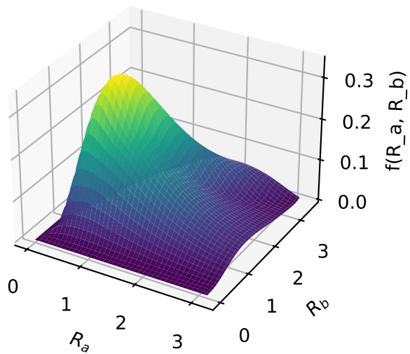
Joint density
