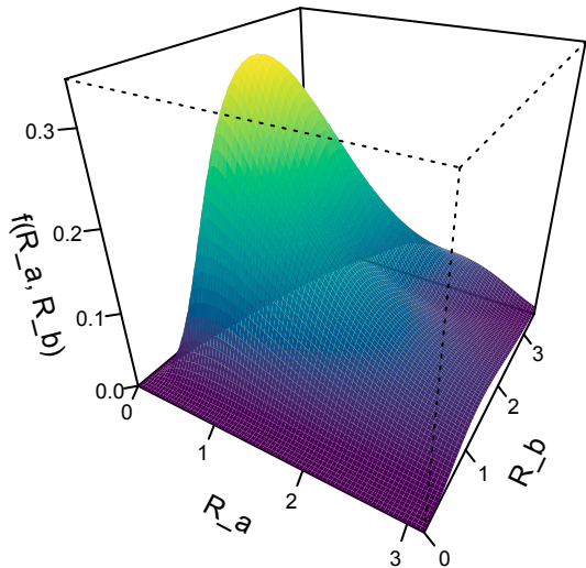
Joint density
