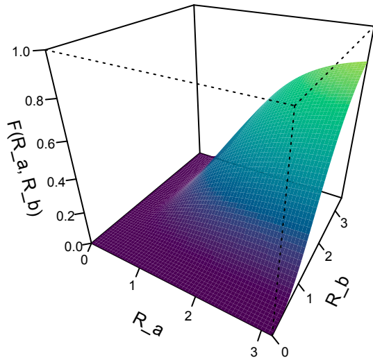
Joint CDF
