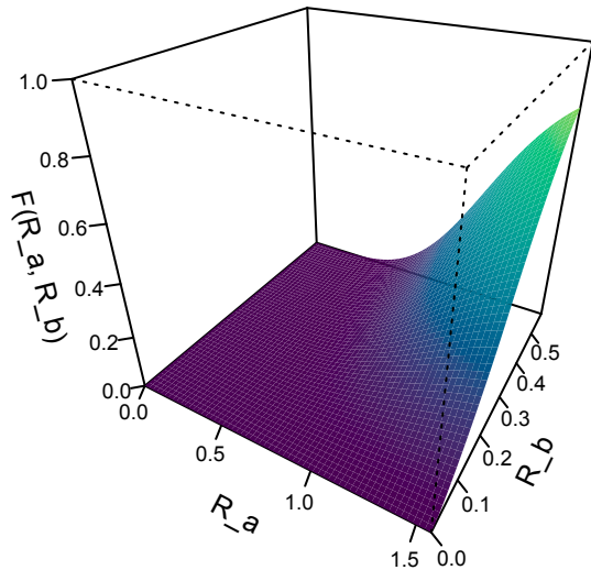
Joint CDF
