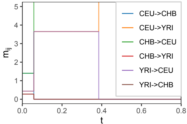
Migration rate trajectory
