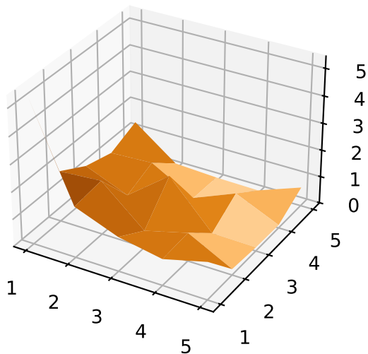
Tightly linked ( r = 0.1 )
