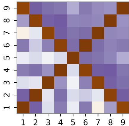
Kingman
