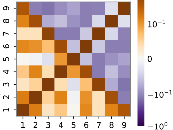
Beta(1.3)
