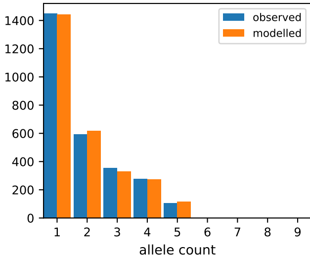
SFS comparison
