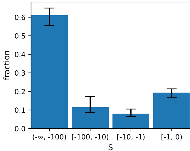
discretized DFE
